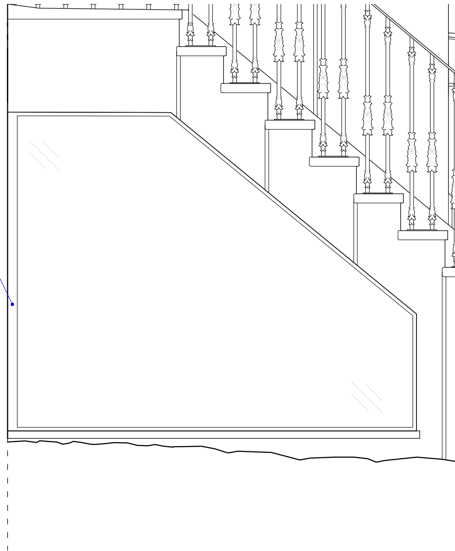
Window 07: Proposed external elevation scale 1:20 @ A3
