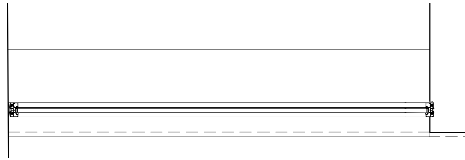
Window 07: Proposed plan scale 1:20 @ A3
