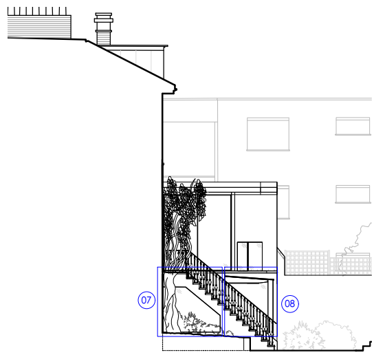
Proposed Side (South) Elevation Location Plan scale 1:200 @ A3
