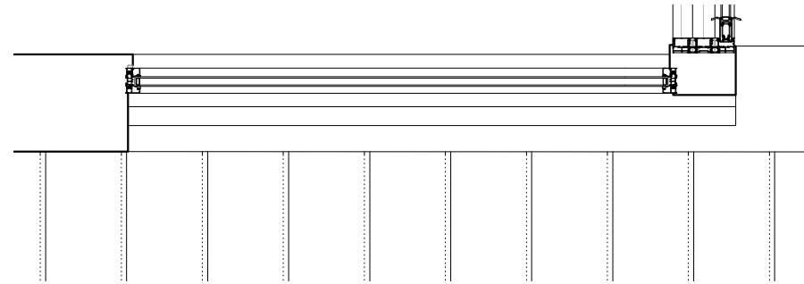
Window 08: Proposed plan scale 1:20 @ A3
