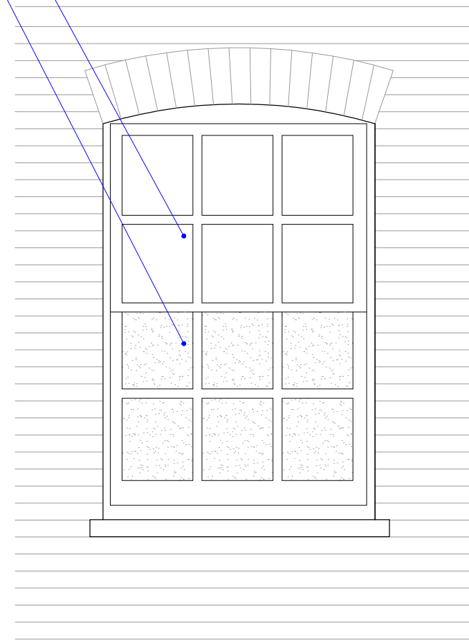
Window 10: Proposed external elevation
