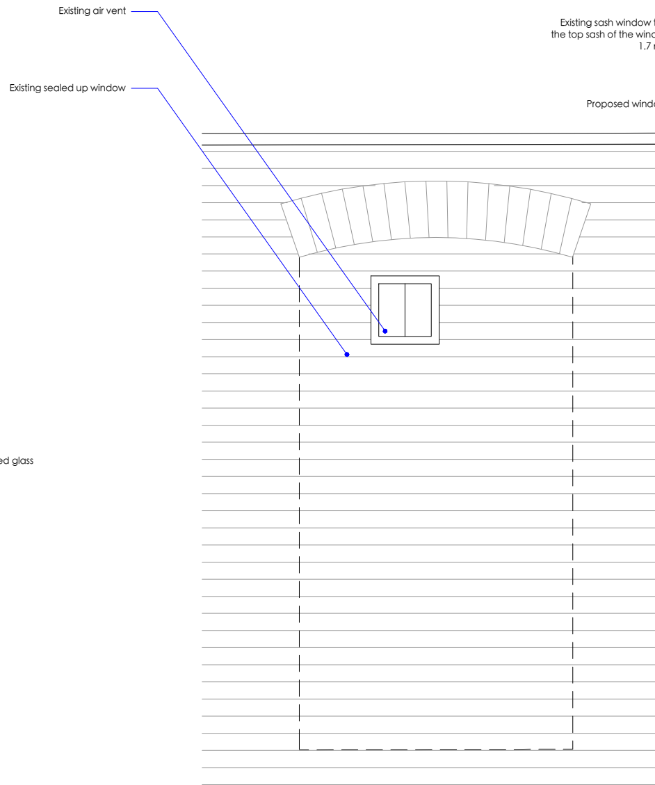
Window 10: Existing external elevation
