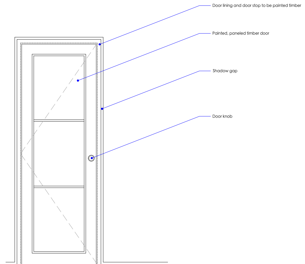
Proposed internal elevation scale 1:20 @ A3
