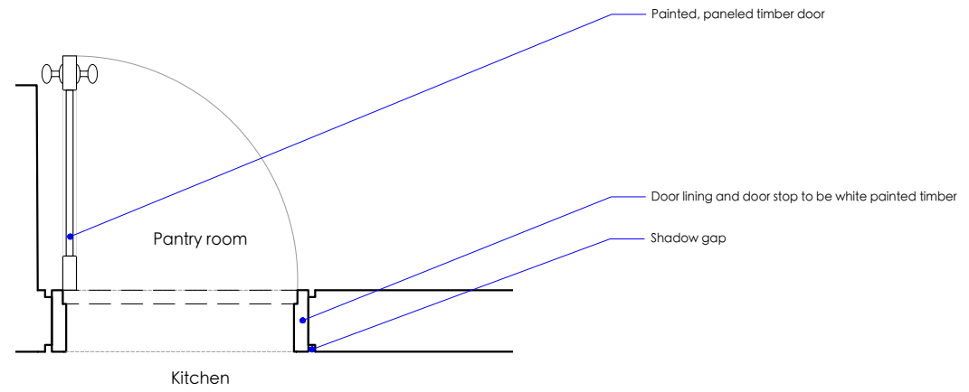
Proposed plan scale 1:20 @ A3
