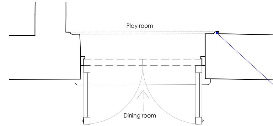
Proposed plan scale 1:20 @ A3
