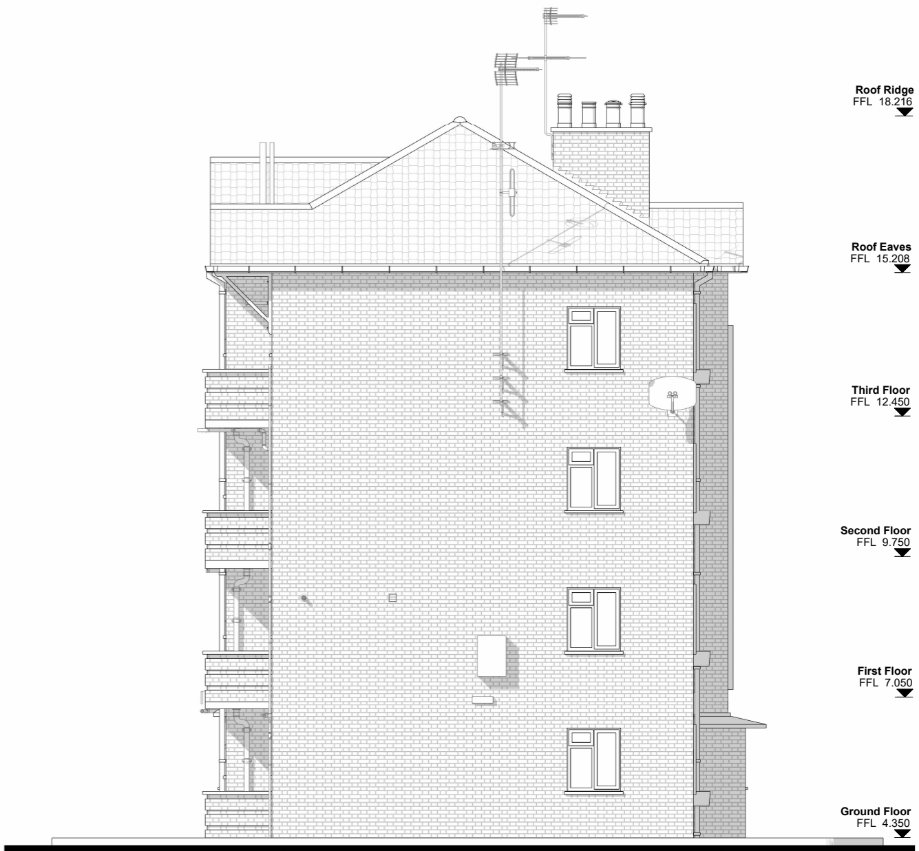
Existing South Side Elevation
