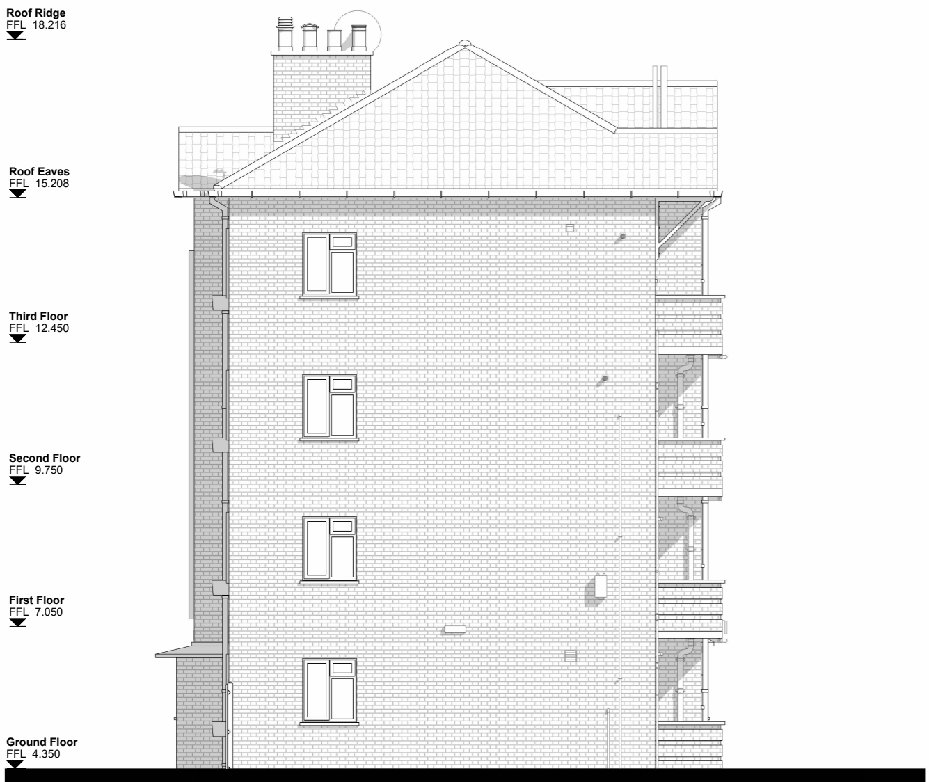
Existing North Side Elevation
