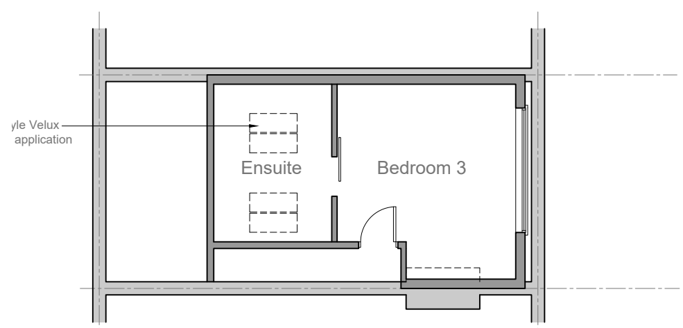
LOFT FLOOR PLAN
