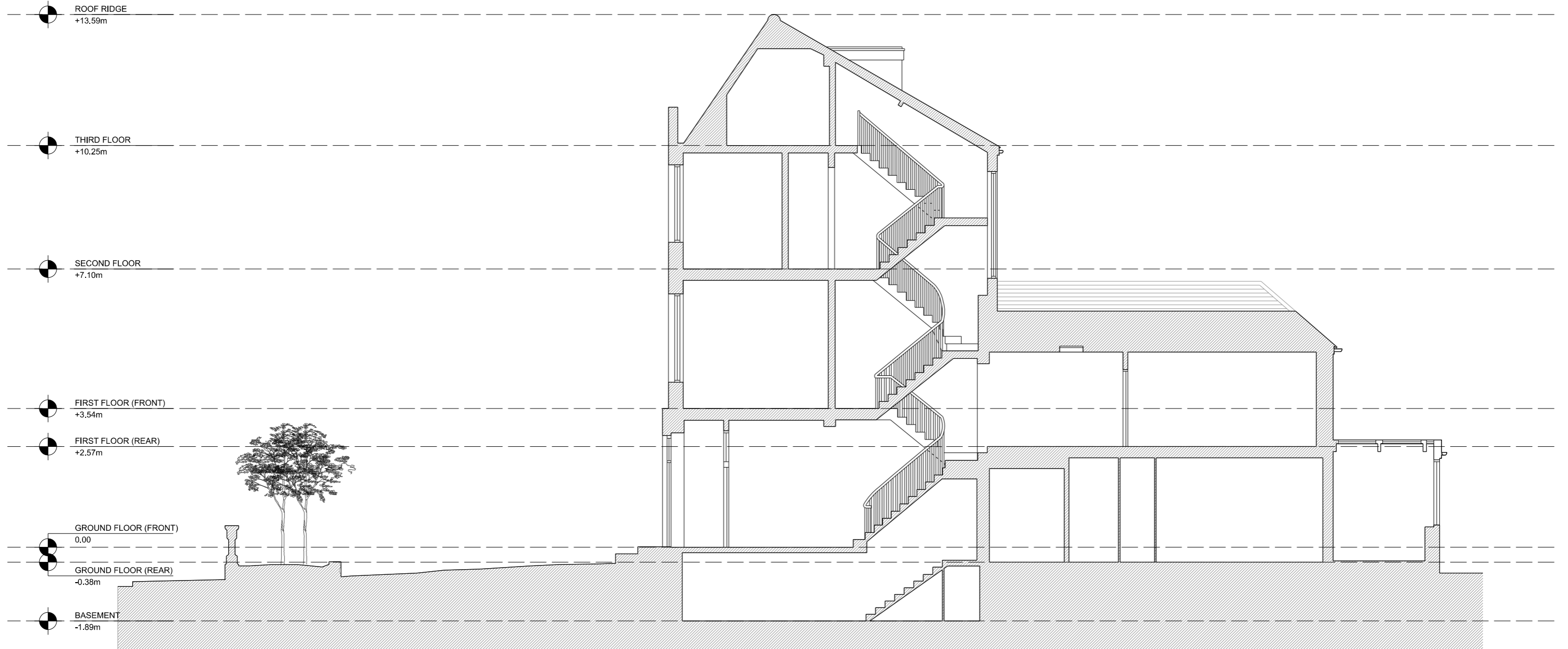
01 EXISTING SECTION AA 1:100
