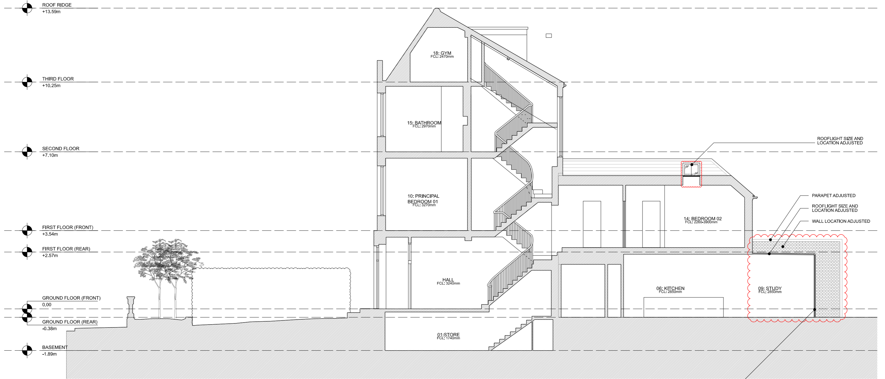
01 PROPOSED SECTION AA 1:100
