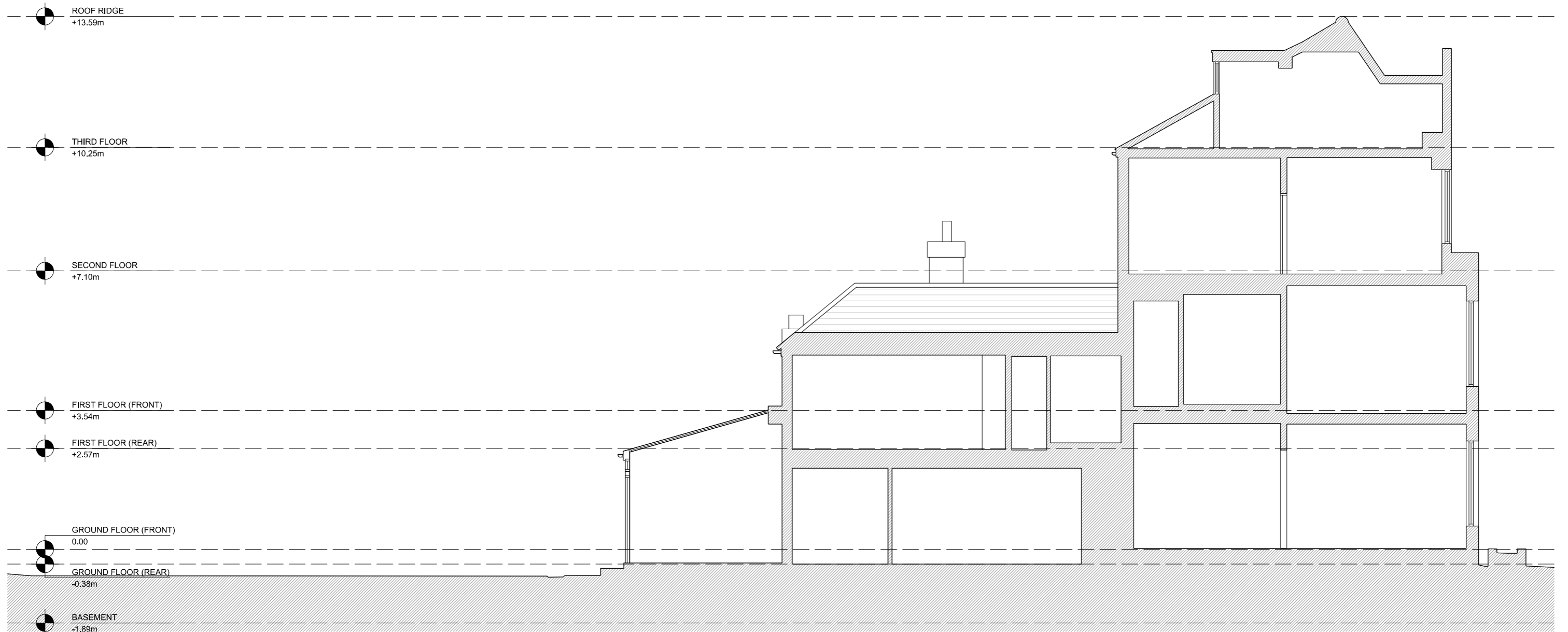
01 EXISTING SECTION CC 1:100
