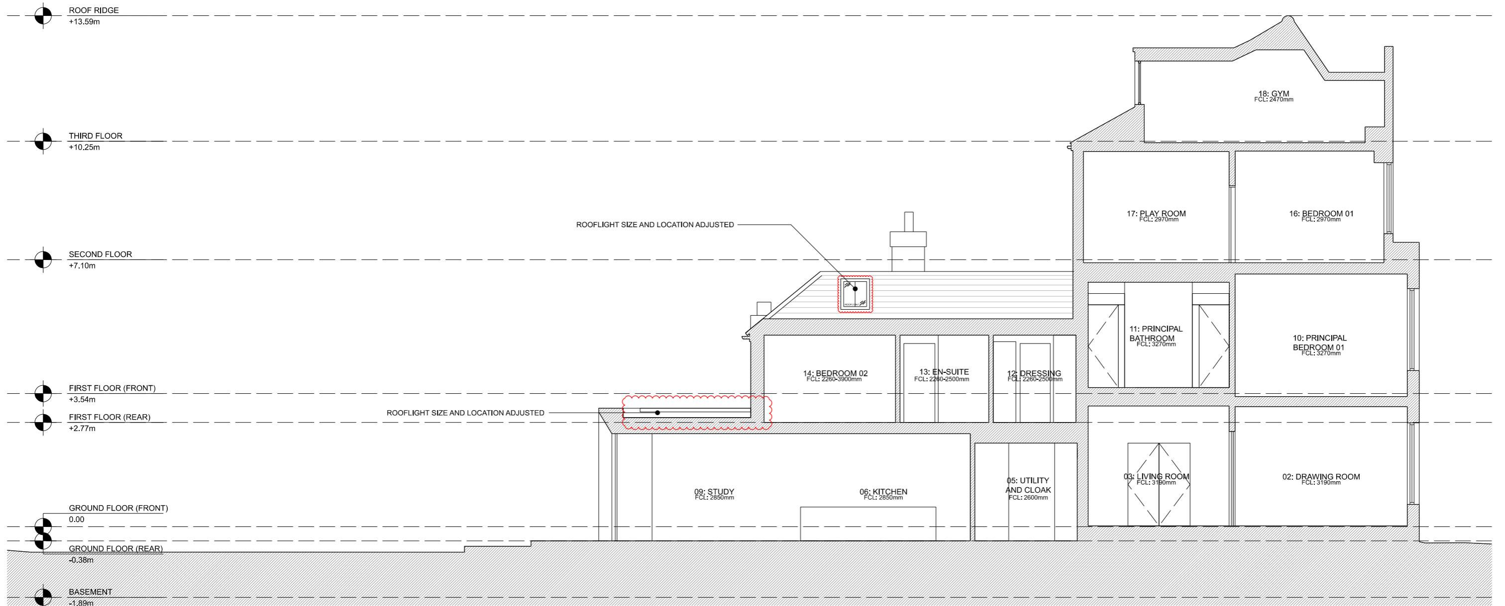
01 PROPOSED SECTION CC 1:100
