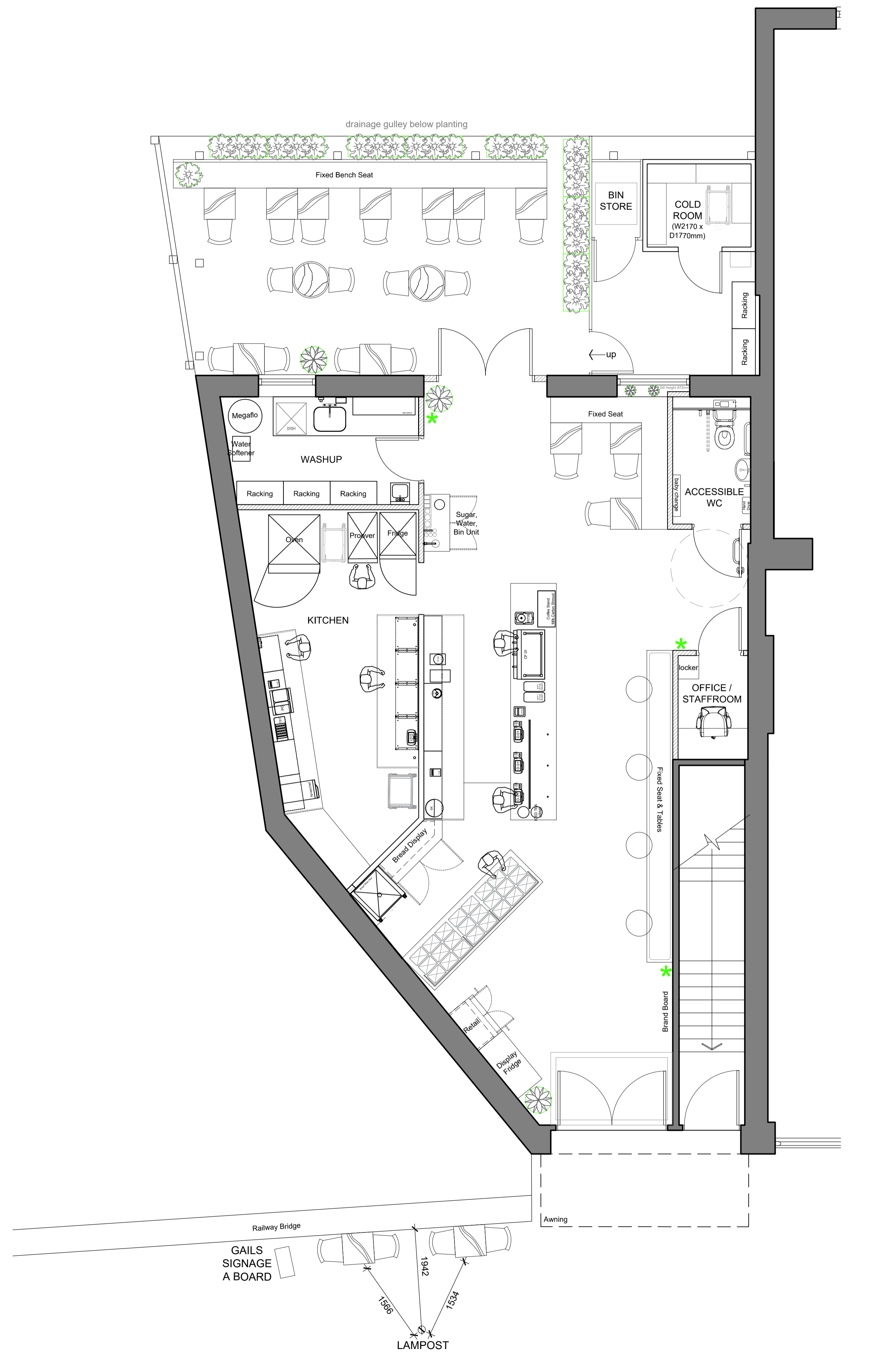
Proposed Plan 1:50
