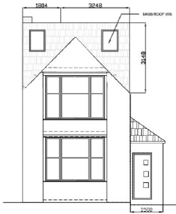
Front Elevation
