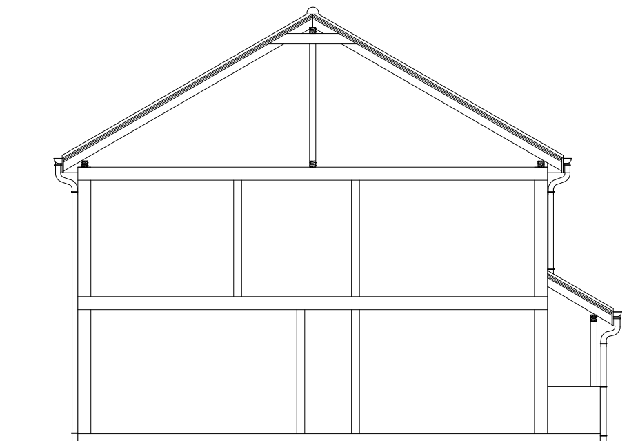
EXISTING LEFT SECTION SCALE 1:100 / A3
