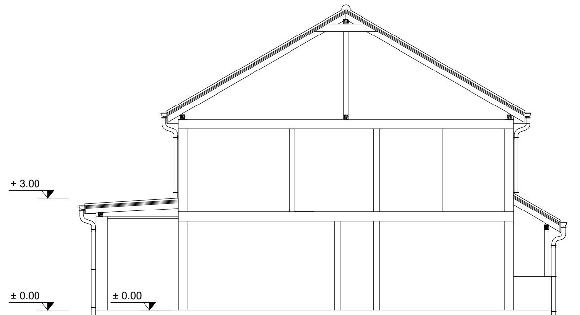
PROPOSED LEFT SECTION SCALE 1:100 / A3
