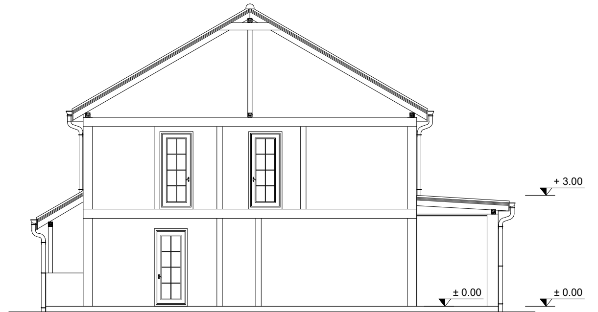
PROPOSED RIGHT SECTION SCALE 1:100 / A3
