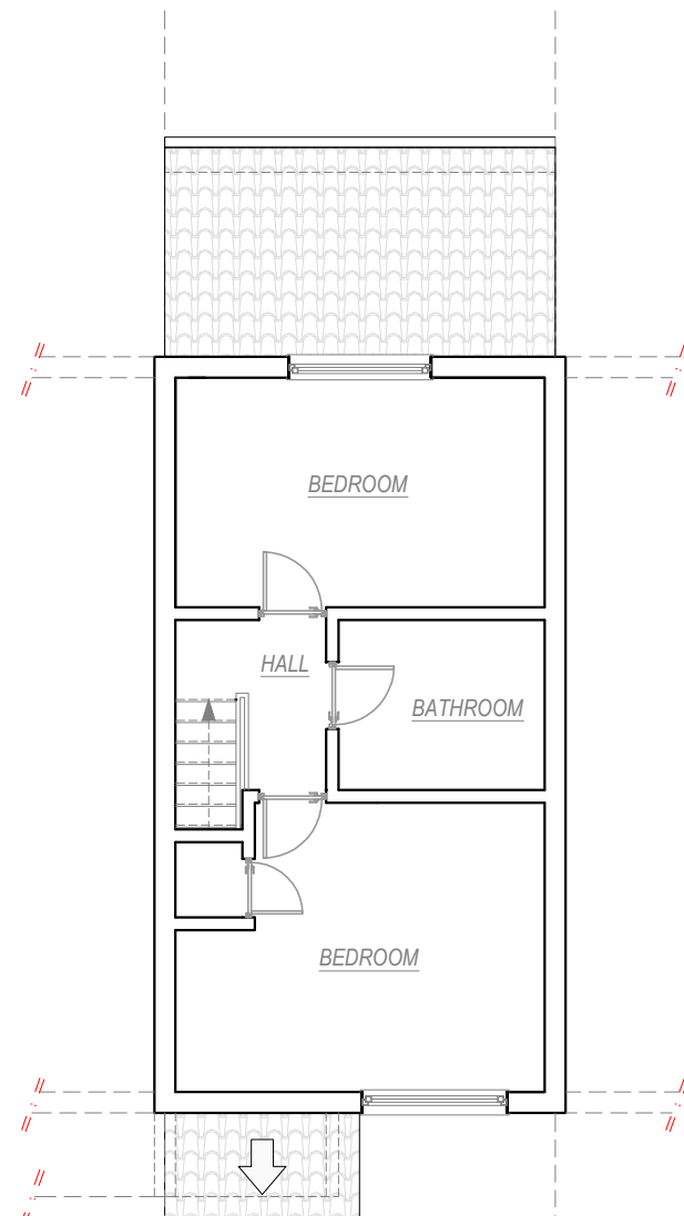
PROPOSED FIRST FLOOR PLAN SCALE 1:100 / A3
