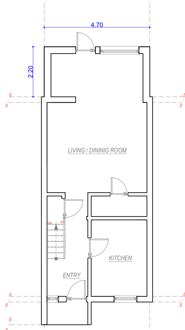
PROPOSED GROUND FLOOR PLAN SCALE 1:100 / A3
