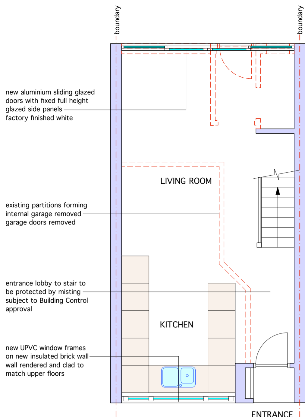
GROUND NEW PROPOSED PLANS
