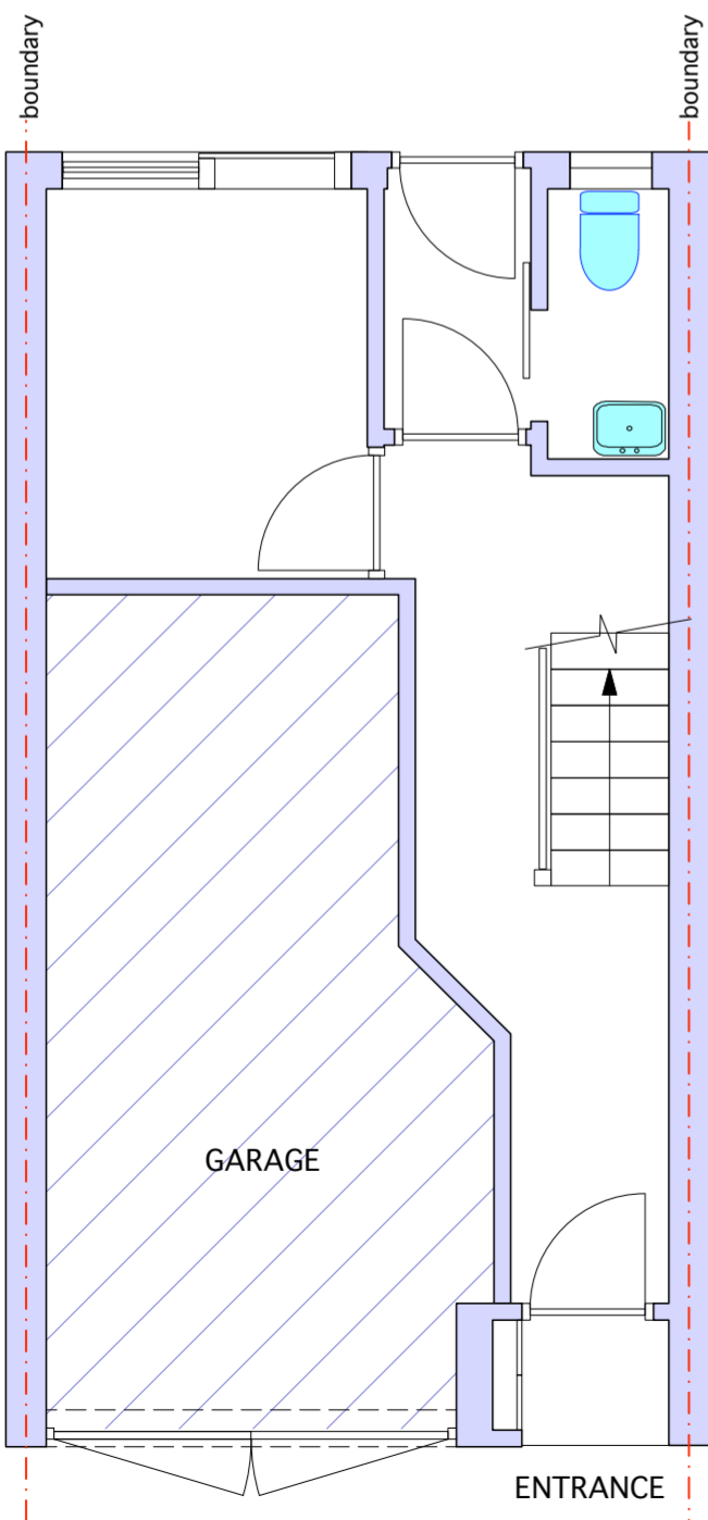
GROUND EXISTING PLANS
