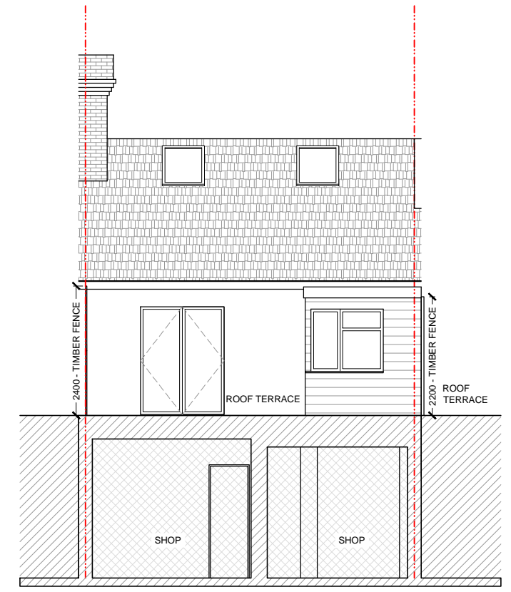
Section B
