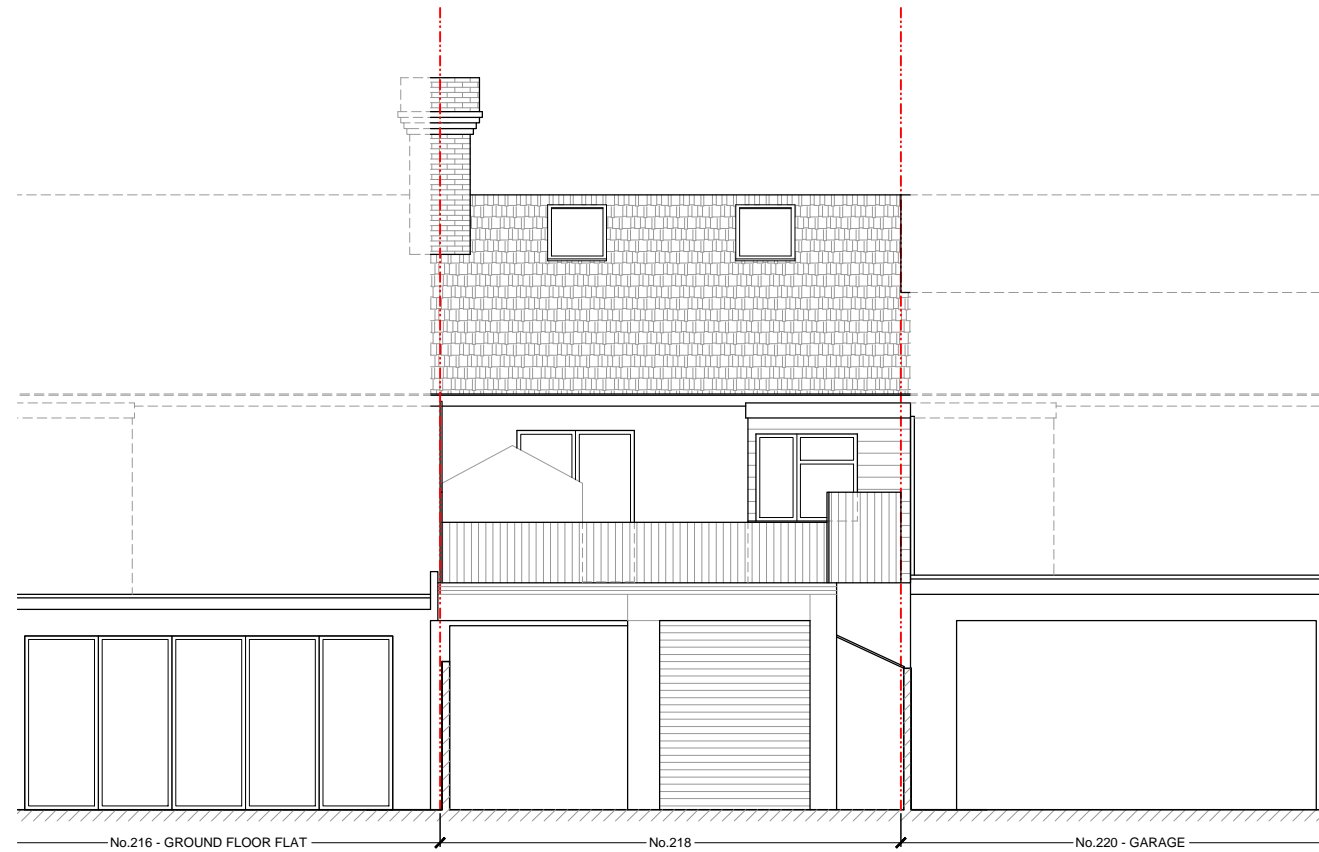
Rear Elevation
