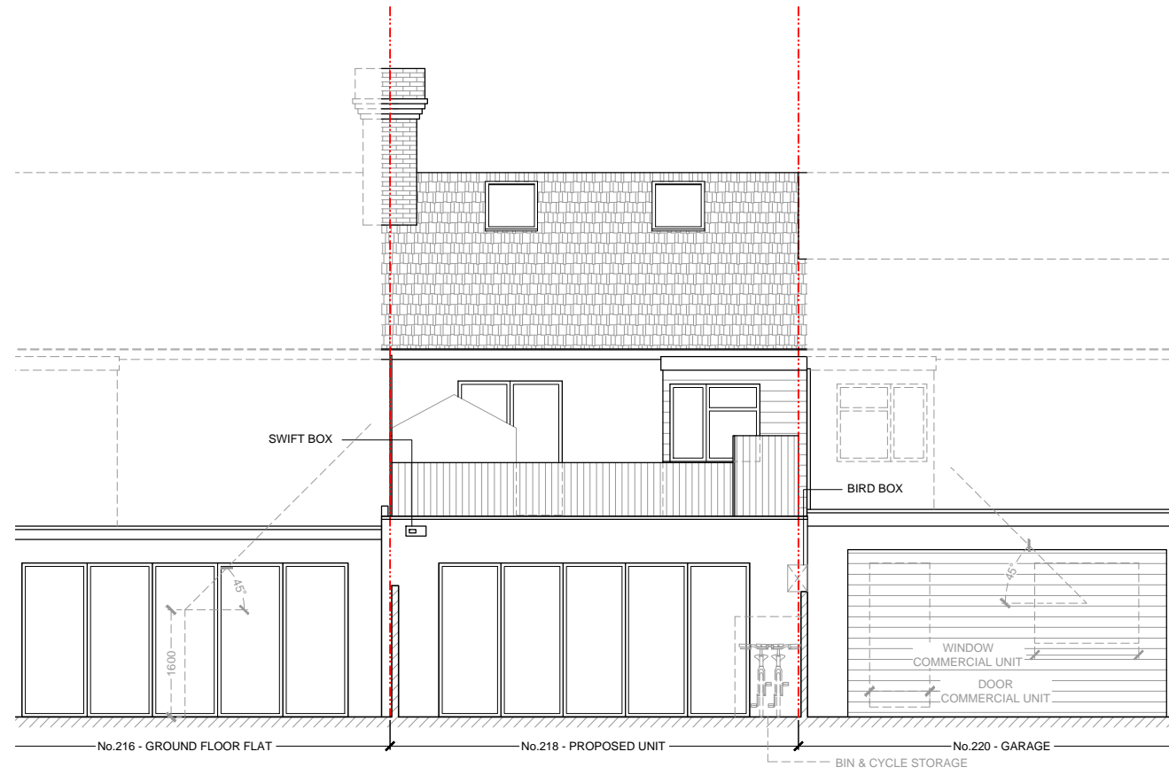
Rear Elevation
