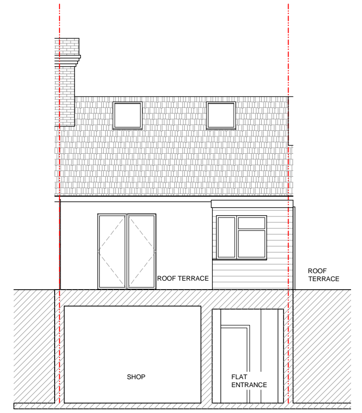
Section B
