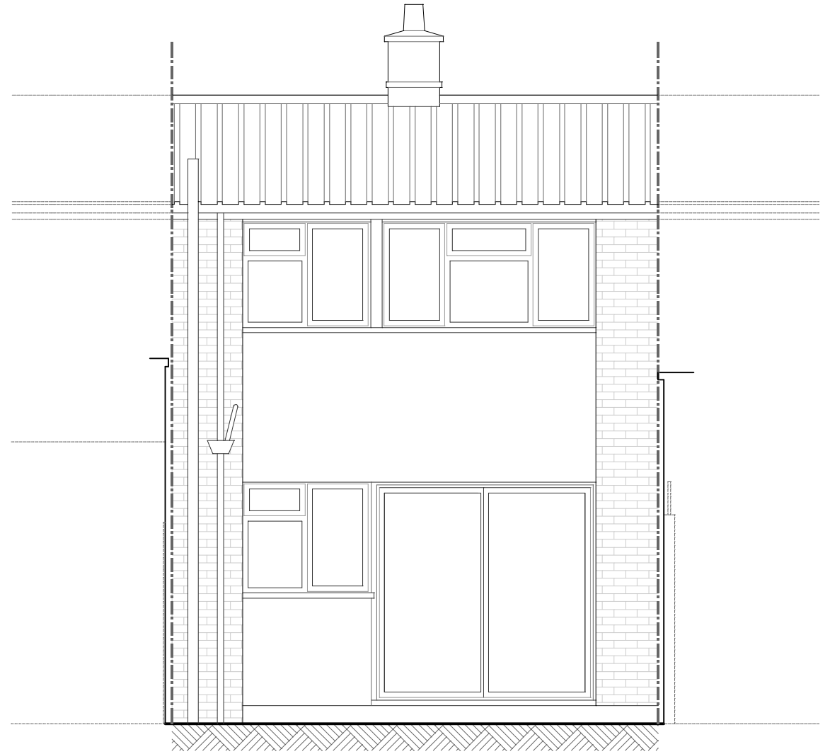
REAR (EAST) ELEVATION
