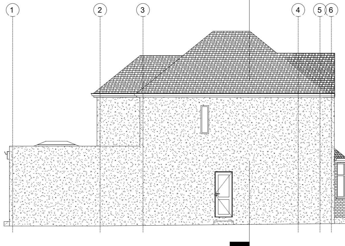
EXISTING LEFT SIDE ELEVATION
