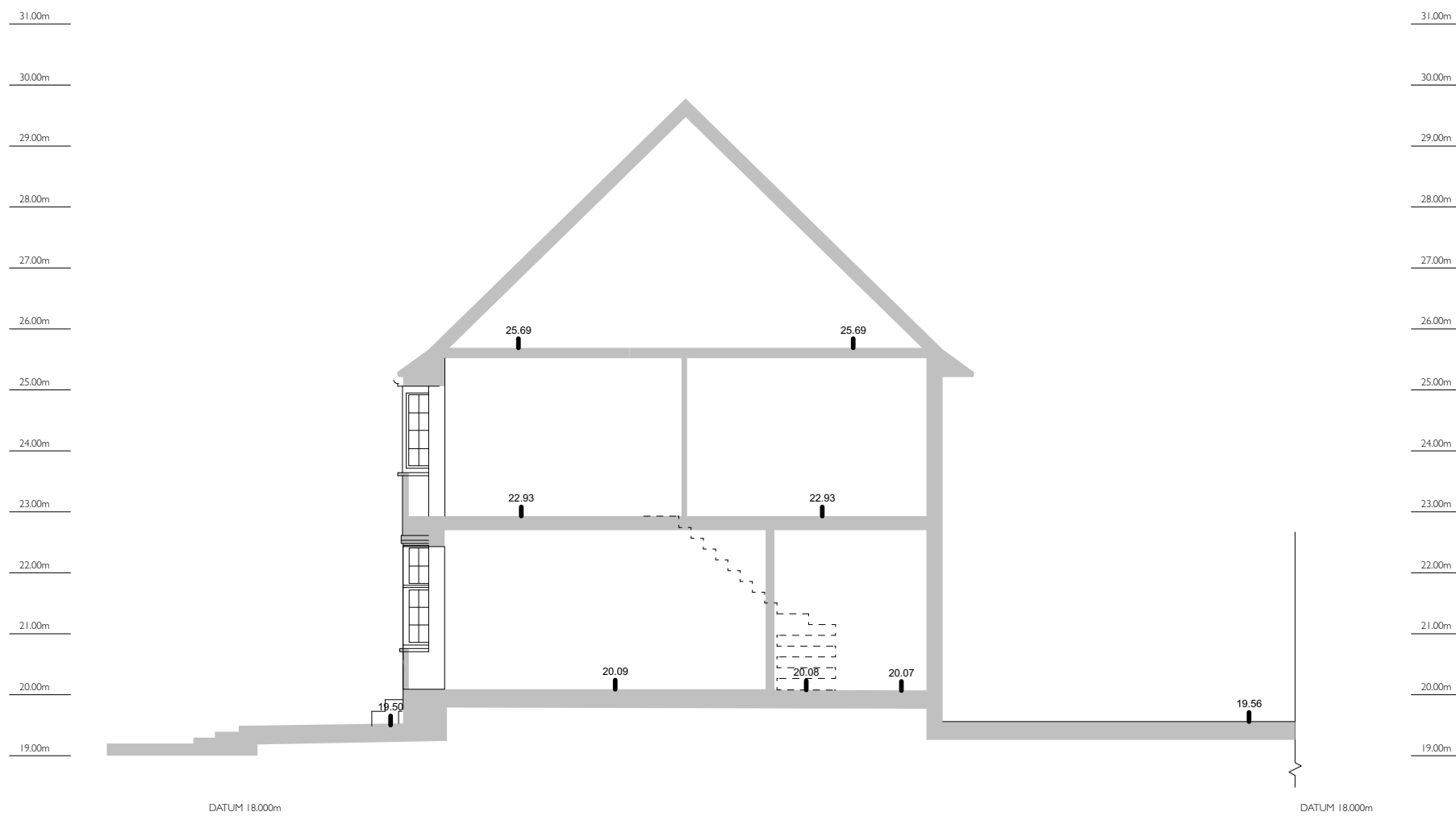
SECTION B-B
