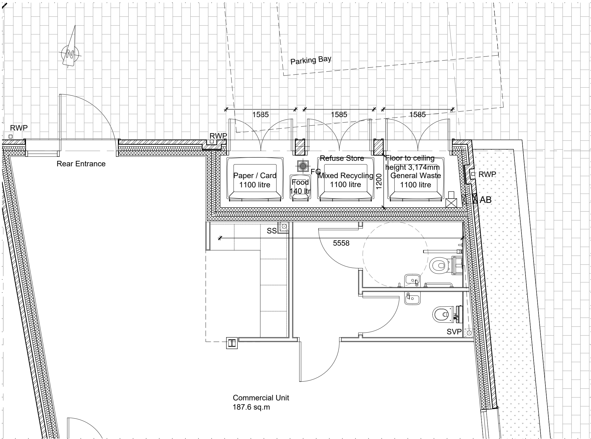
Extract of Block B Ground Floor GA Plan showing Block B Refuse Store
