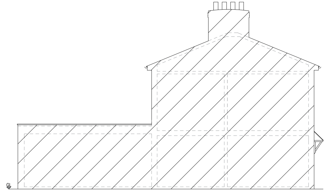
Side (N/E) Elevation Existing
