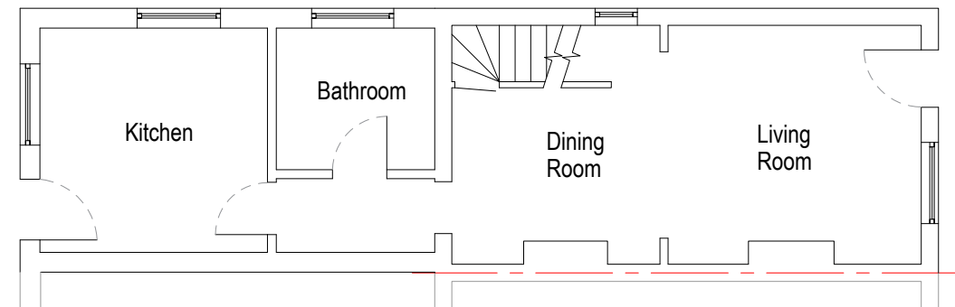
Ground Floor Existing
