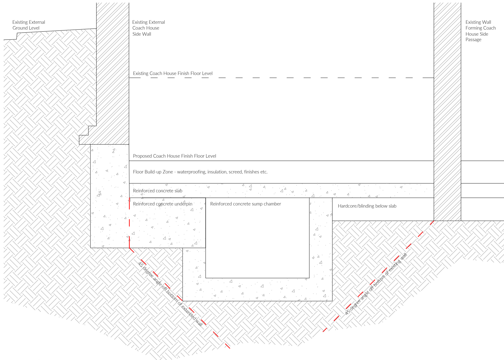
122 Castelnau - SK01 Sketch Section Through Coach House Showing Location of Sump Chamber in Relation to Foundations 1:20 @ A4 29 08 2024
