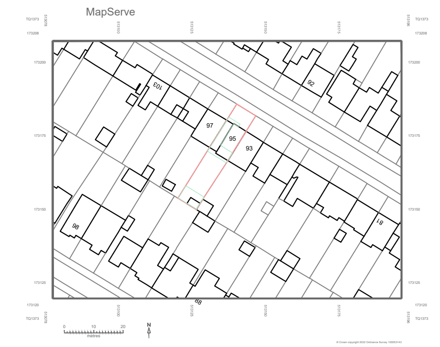
Site Location Plan 1:1250 @A1
