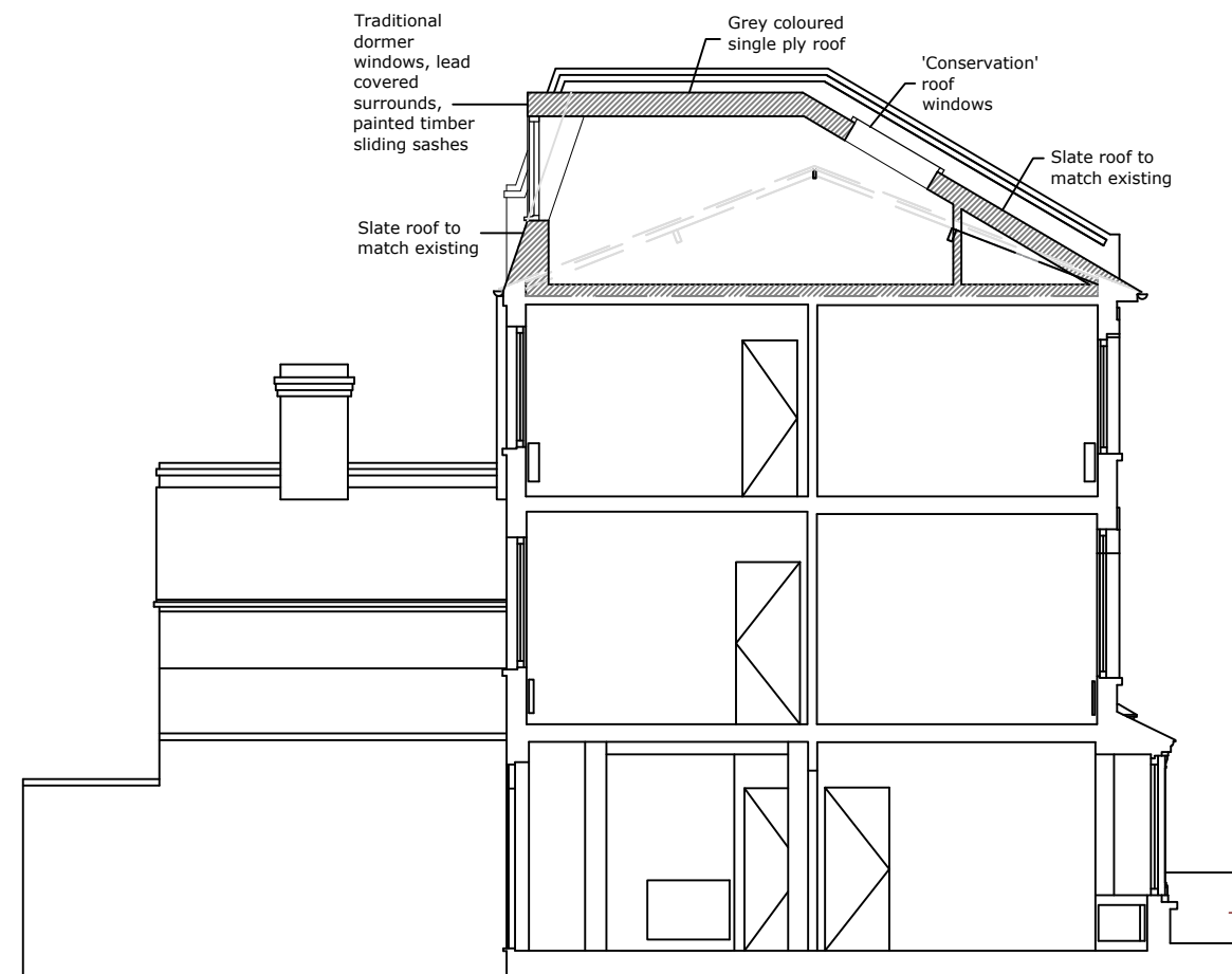
PROPOSED SECTION AA/SIDE ELEVATION
