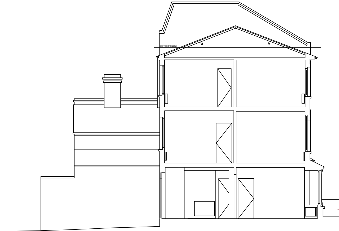
EXISTING SECTION AA/SIDE ELEVATION
