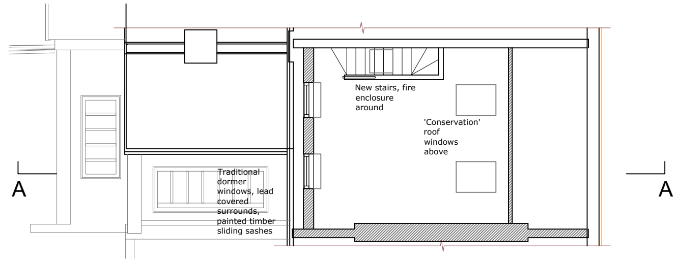
ROOF EXTENSION FLOOR PLAN
