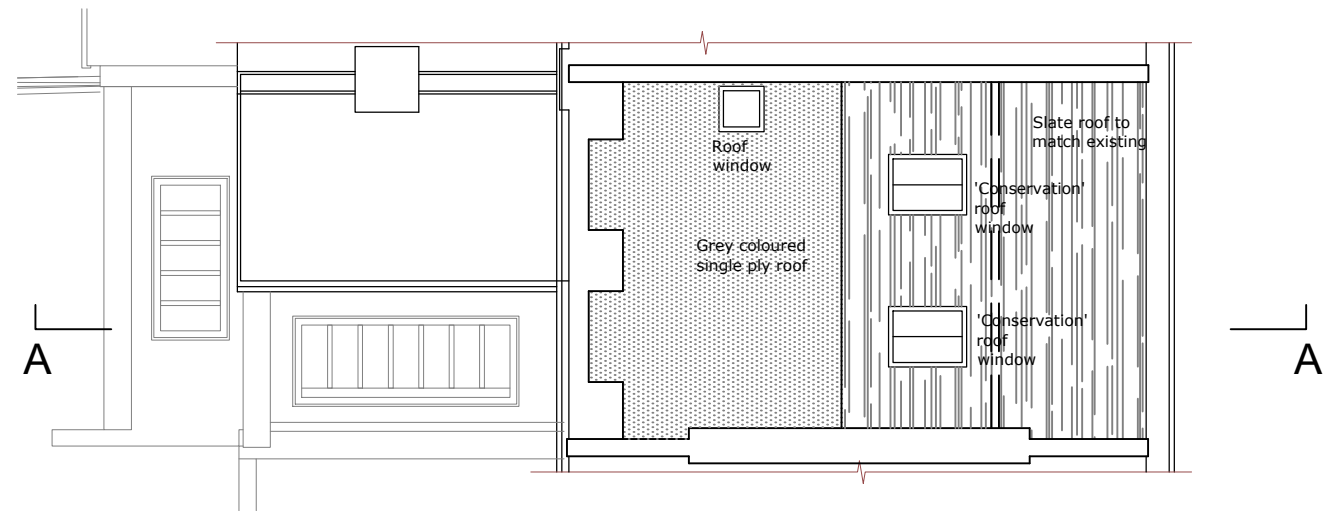
ROOF PLAN
