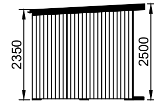
Left Elevation
