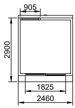
Floor Plan
