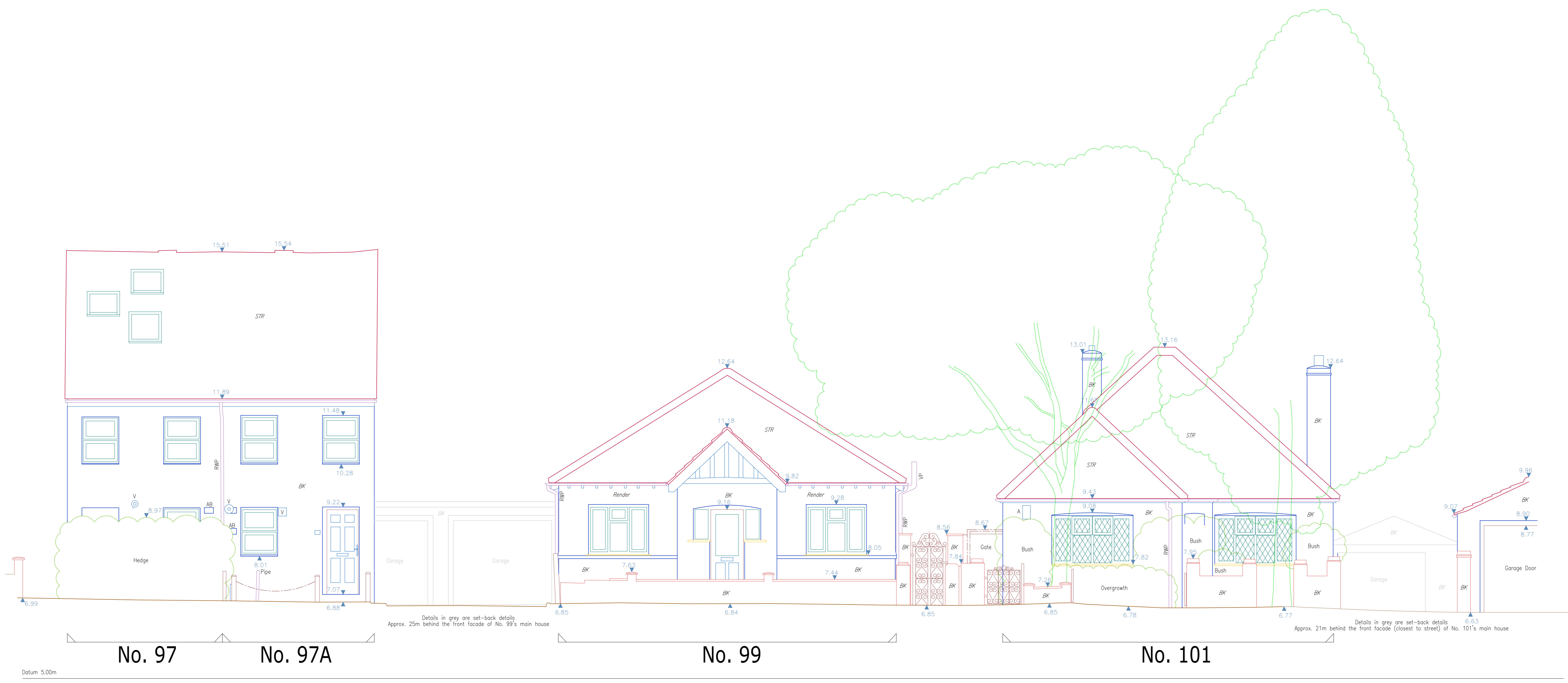
Street Scene Elevation
