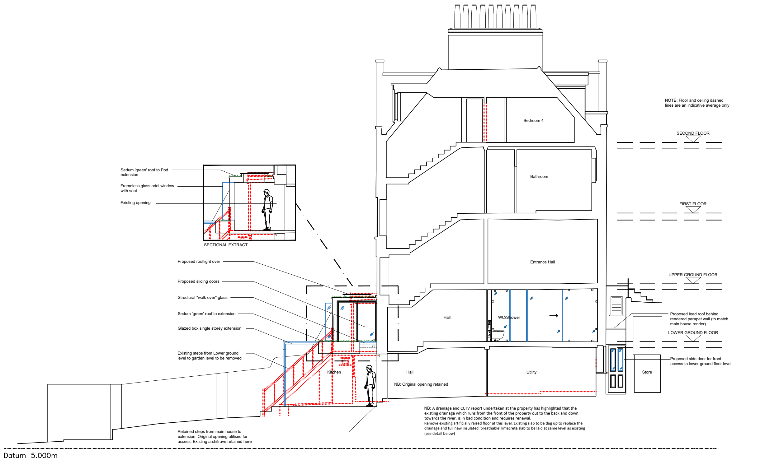
Proposed Section AA 1:100@A3
