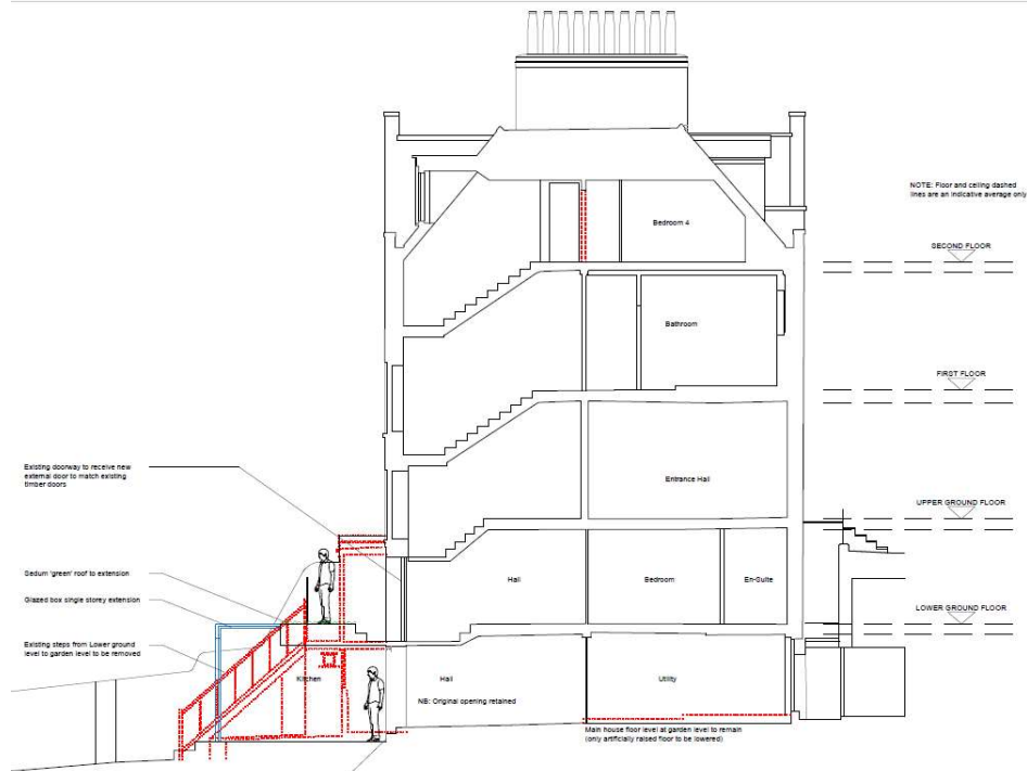
Proposed Section Plan
