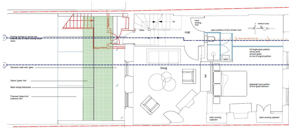
Proposed Lower Ground Floor Plan
