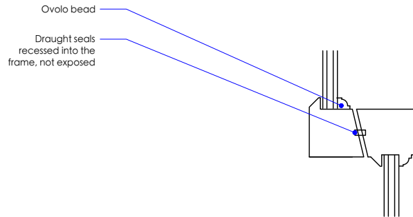
D3 - Meeting Rail Detail scale 1:5 @ A4
