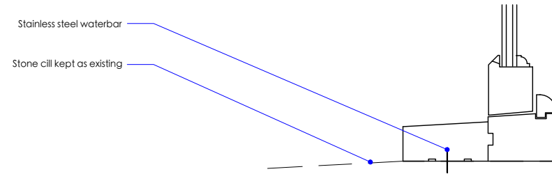
D4 - Sash window cill detail scale 1:5 @ A4
