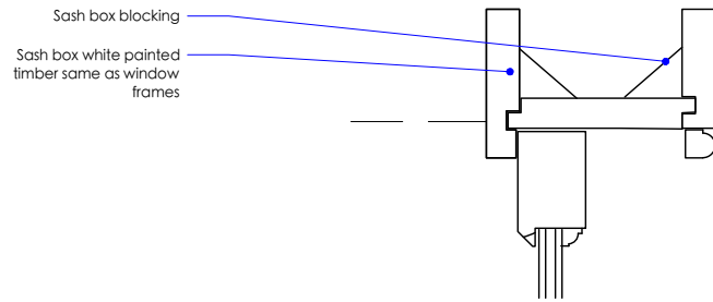
D1 - Sash window head detail scale 1:5 @ A4
