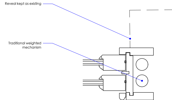
D5 - Sash window jamb detail scale 1:5 @ A4
