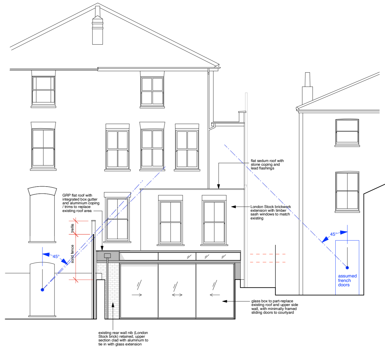
REAR ELEVATION
