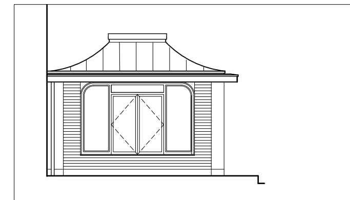
PROPOSED SIDE ELEVATION south Dining room extension.
