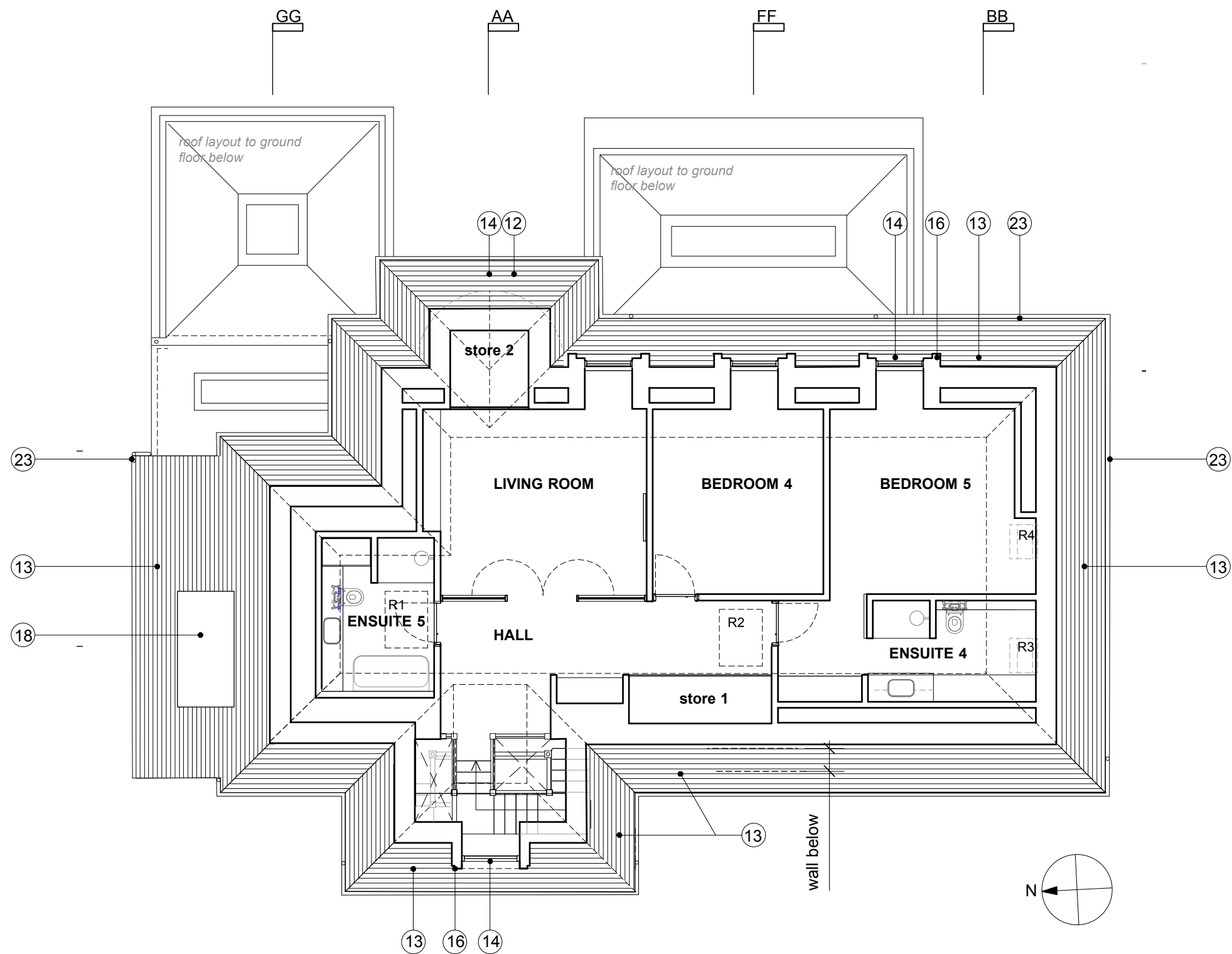
PROPOSED LOFT FLOOR PLAN
