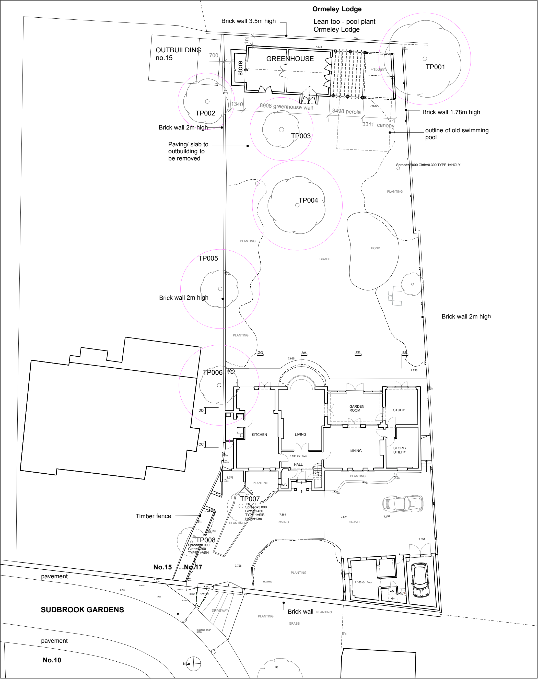
PROPOSED BLOCK PLAN 1:200 @A3, 1:100 @A1
