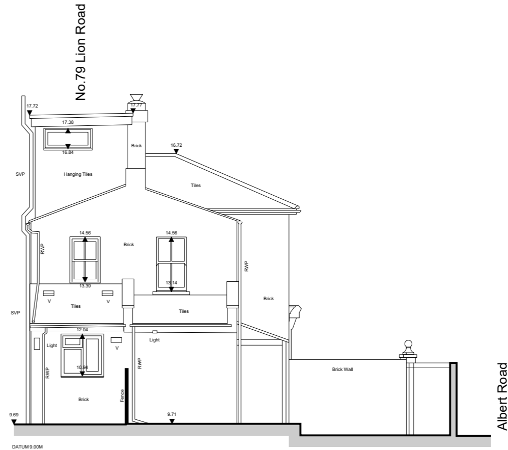
EXISTING NORTH ELEVATION
