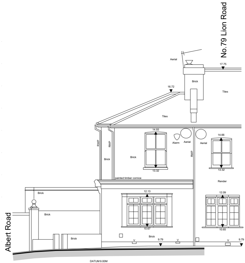
EXISTING SOUTH ELEVATION
