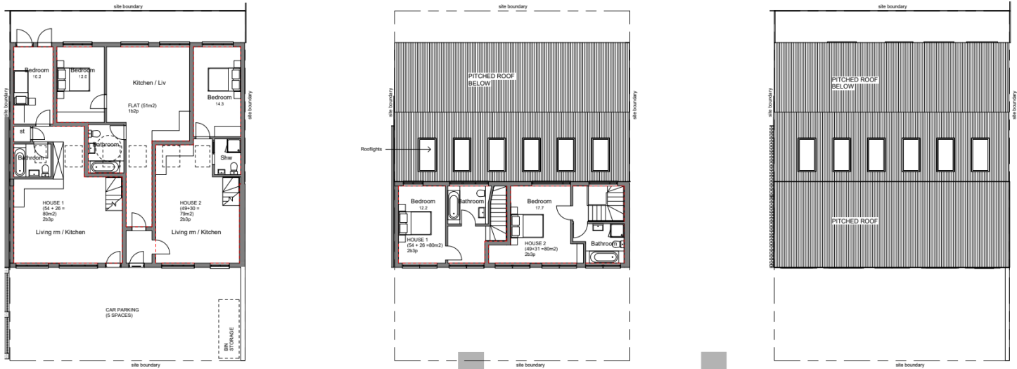
Figure 6: Proposed floor plans
