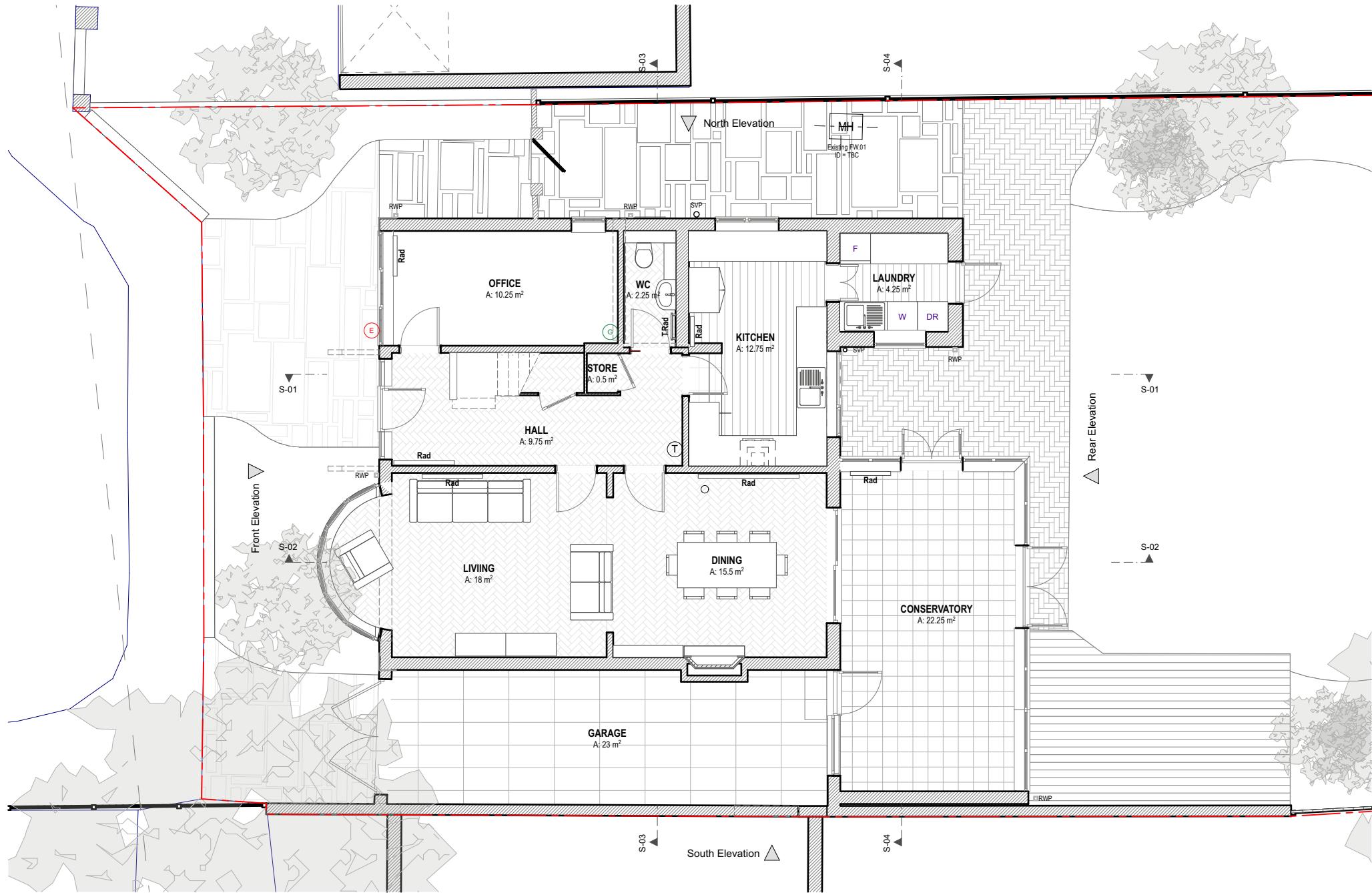
Ground Floor
