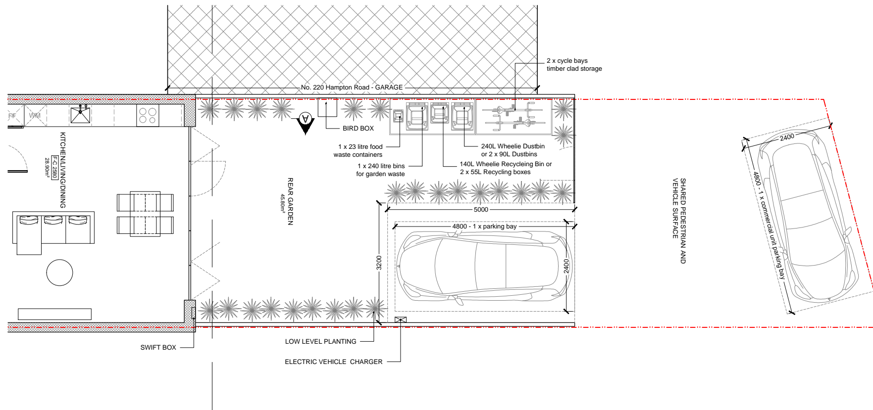
Ground Floor Plan - part 2
