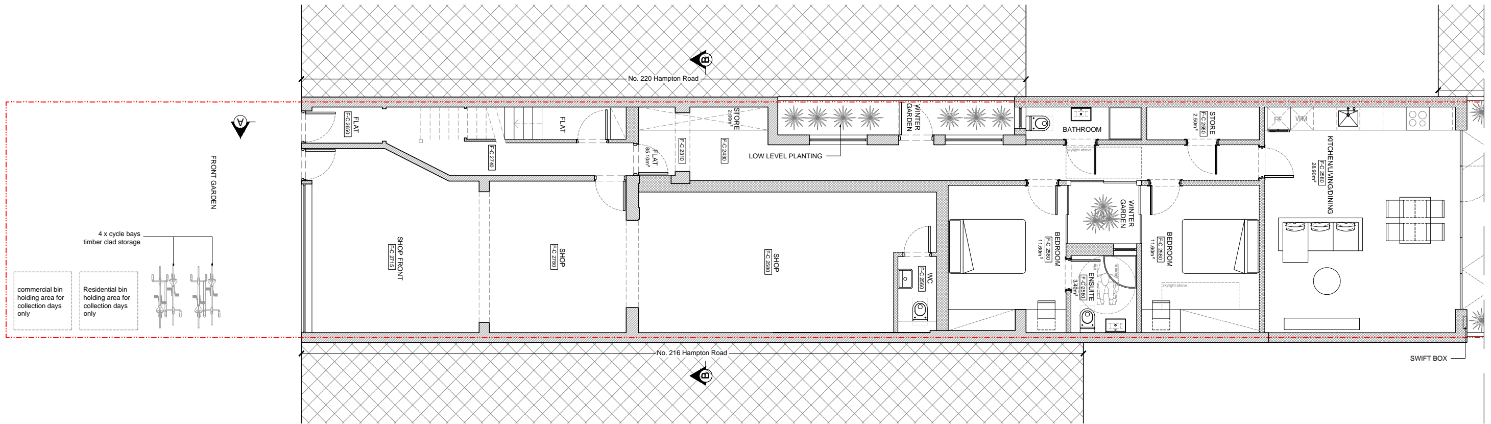
Ground Floor Plan - part 1
