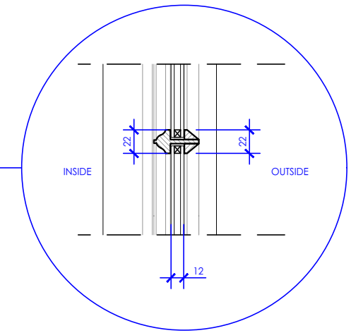
Proposed Sash Window Detail Section scale 1:5
