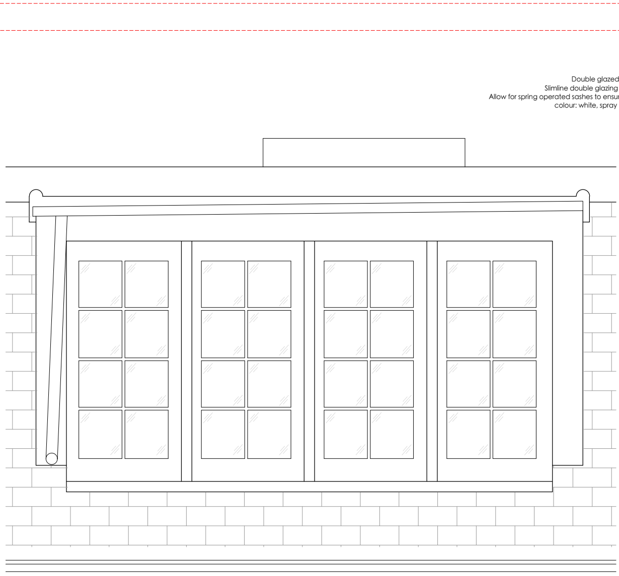
Window 04: Proposed external elevation (front and rear dormers are identical) scale 1:20 @ A3
