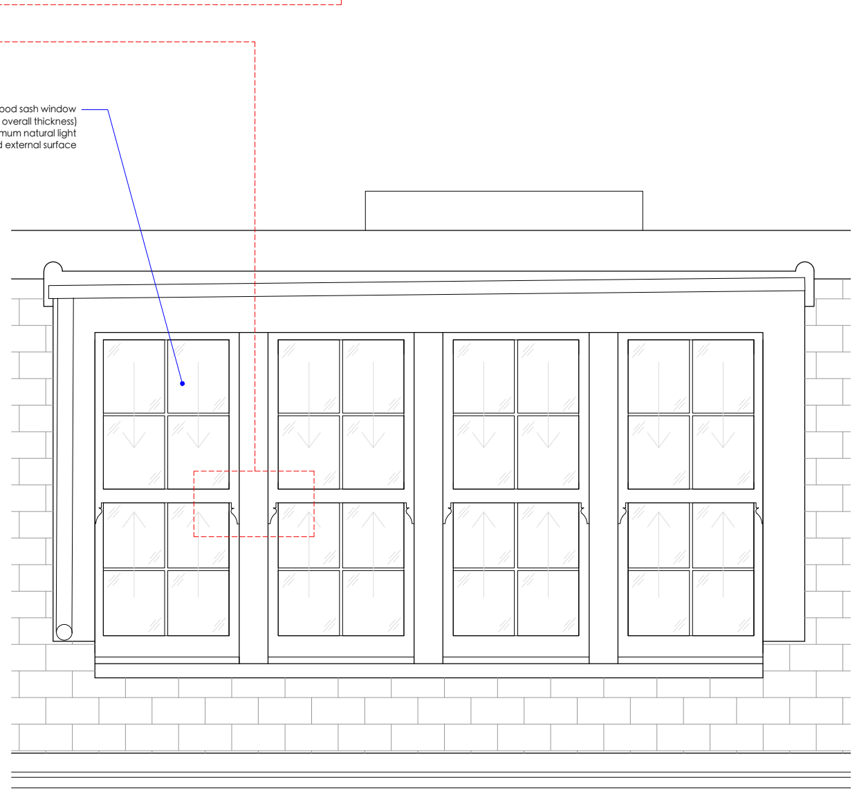
Window 04: Proposed external elevation identical in both rear and front proposed dormers) scale 1:20 @ A3
