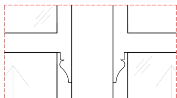
Close up detail of proposed horns scale 1:10 @ A3
