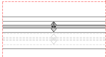
Close up detail of structural glazing bars scale 1:10 @ A3
