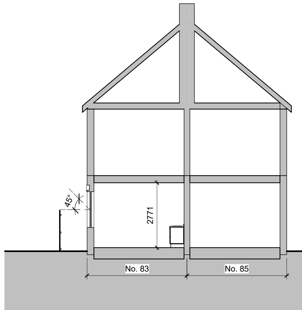
PROPOSED SECTION 1 : 100
