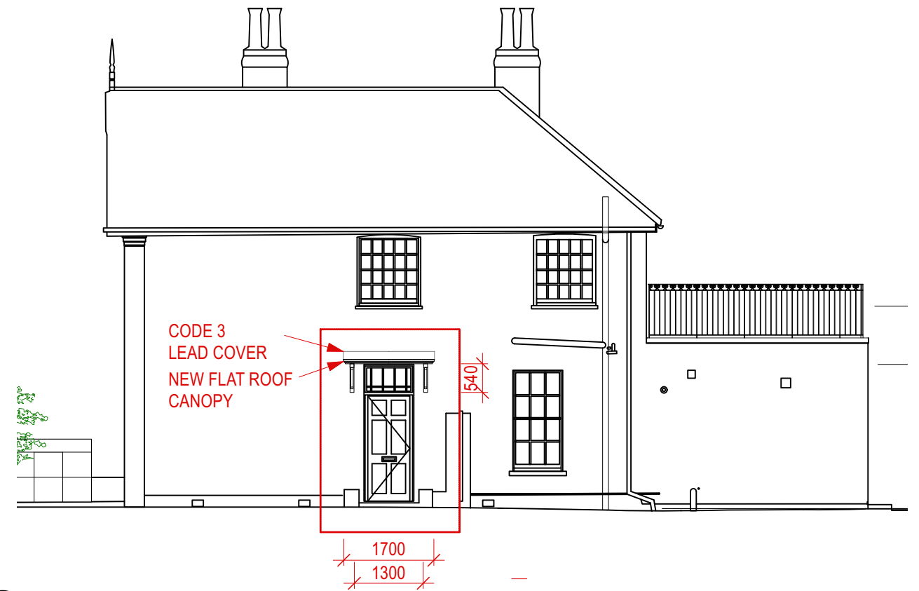
1 EAST ELEVATION AS PROPOSED 1:100
