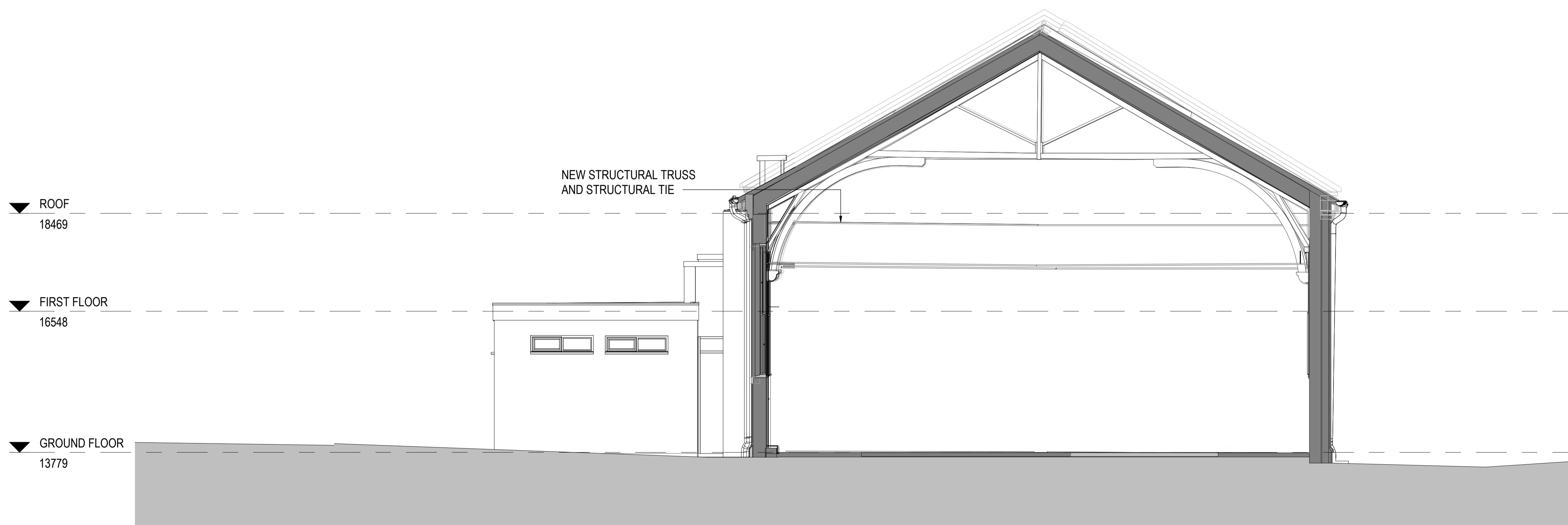
2 SHORT SECTION BB - PROPOSED 1 : 50
