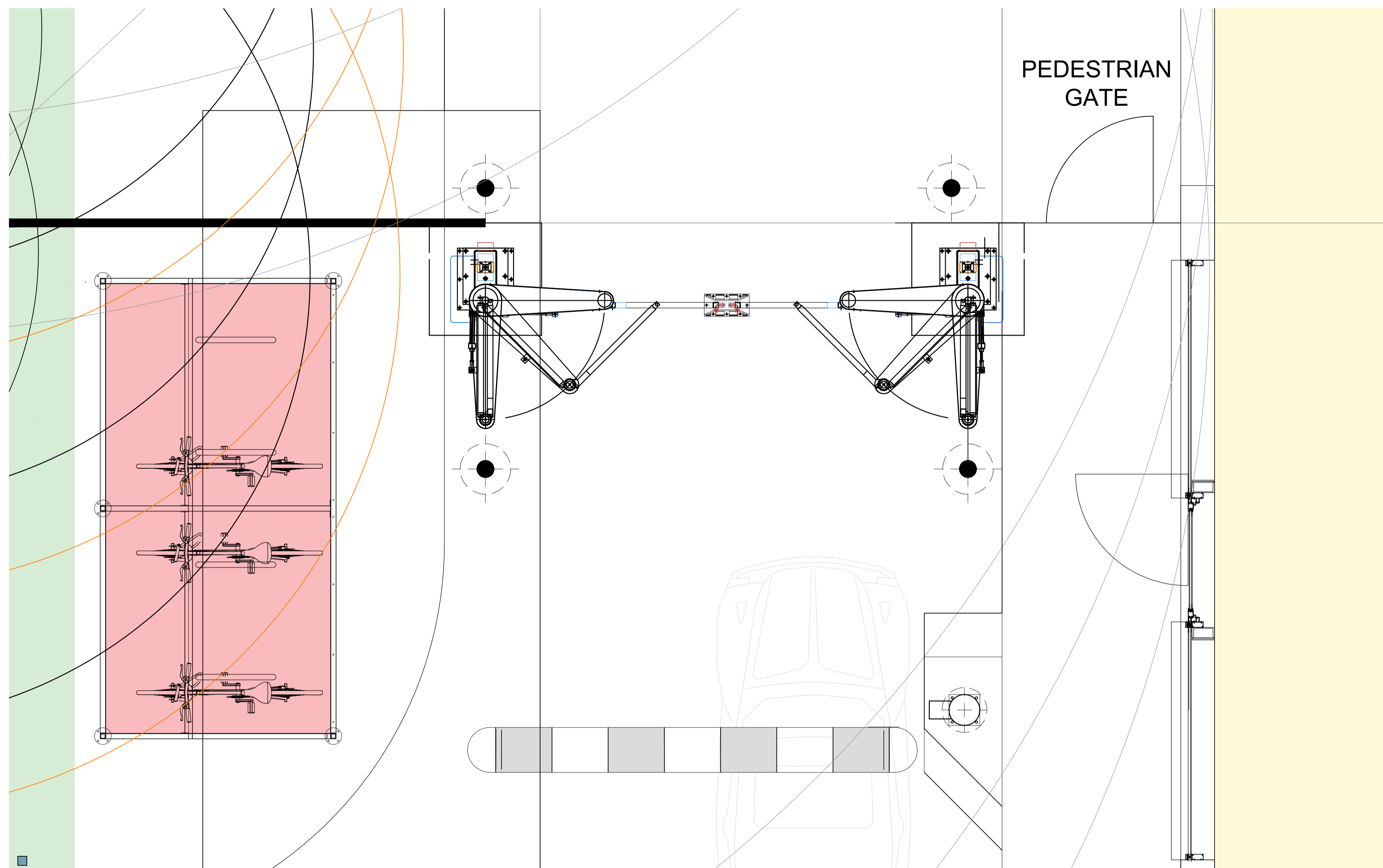
SECURITY BI-FOLDING GATE PLAN AS PROPOSED SCALE 1:25
