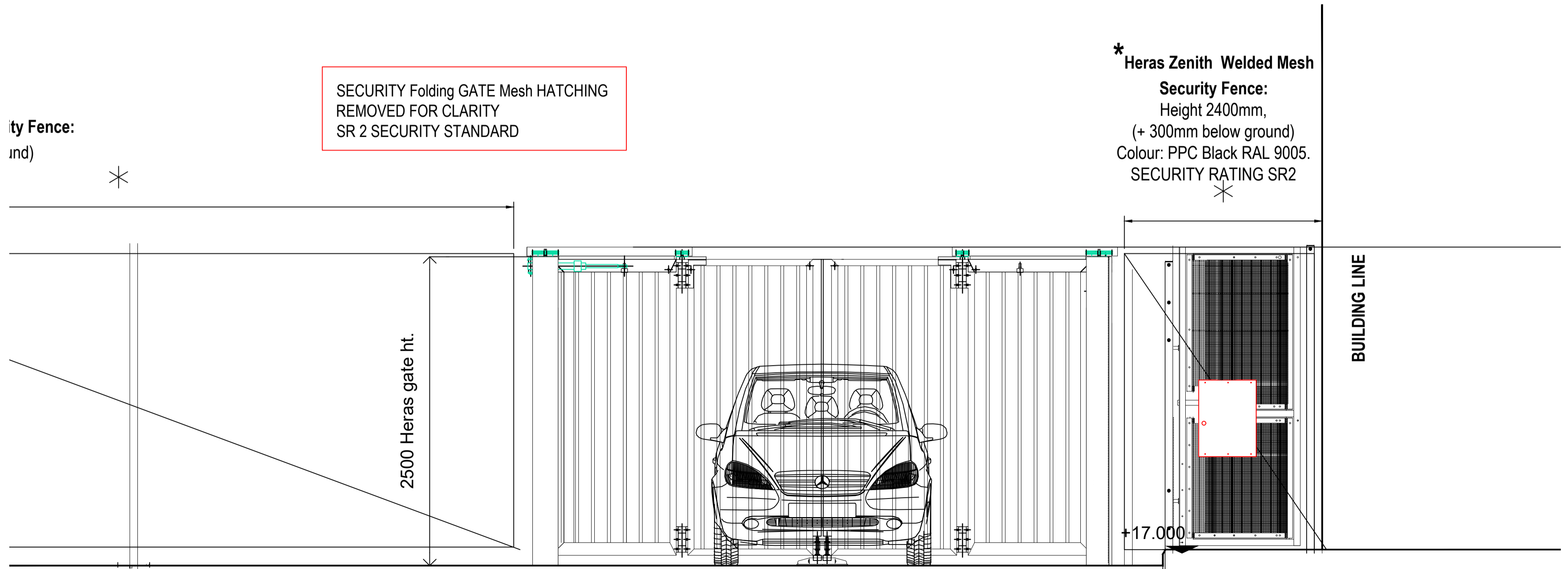
SECURITY BI-FOLDING GATE ELEVATION AS PROPOSED SCALE 1:25 SR 2 SECURITY STANDARD
