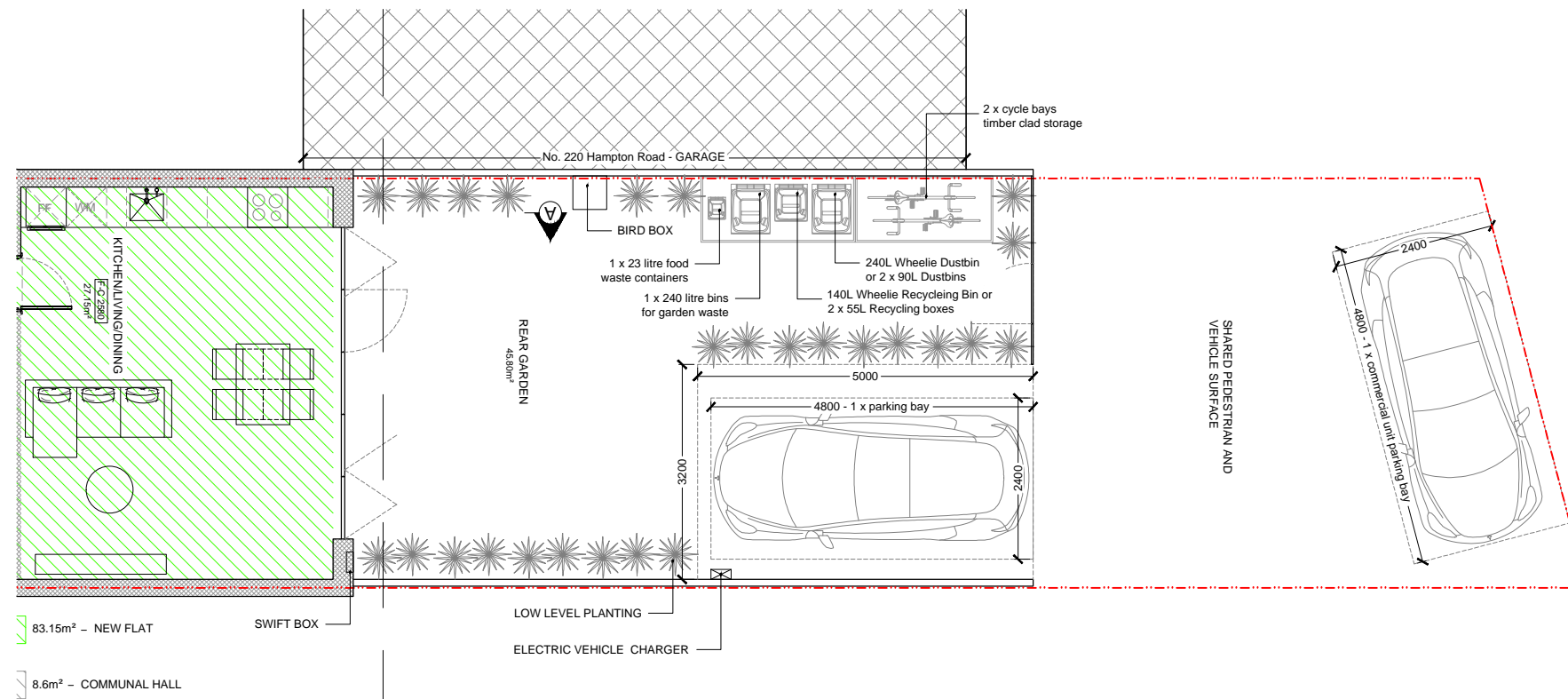
Ground Floor Plan - part 2
