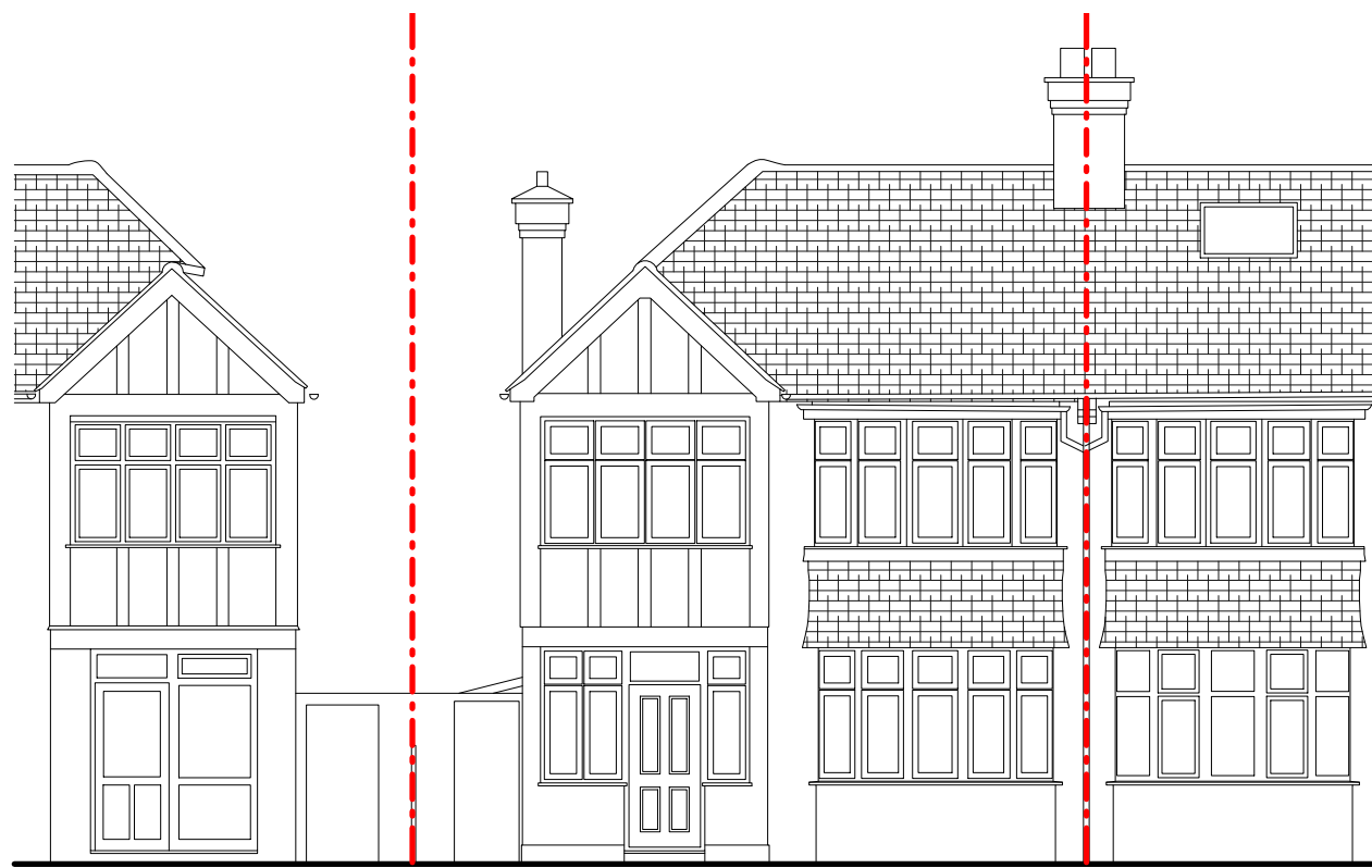
Existing Front Elevation 1 : 100
