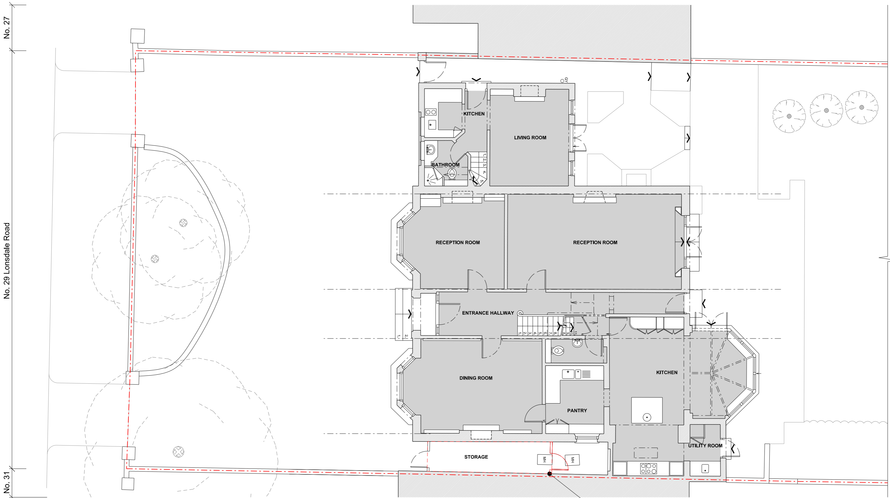
01 Demolition Ground Floor Plan 1:100 Front Garden
