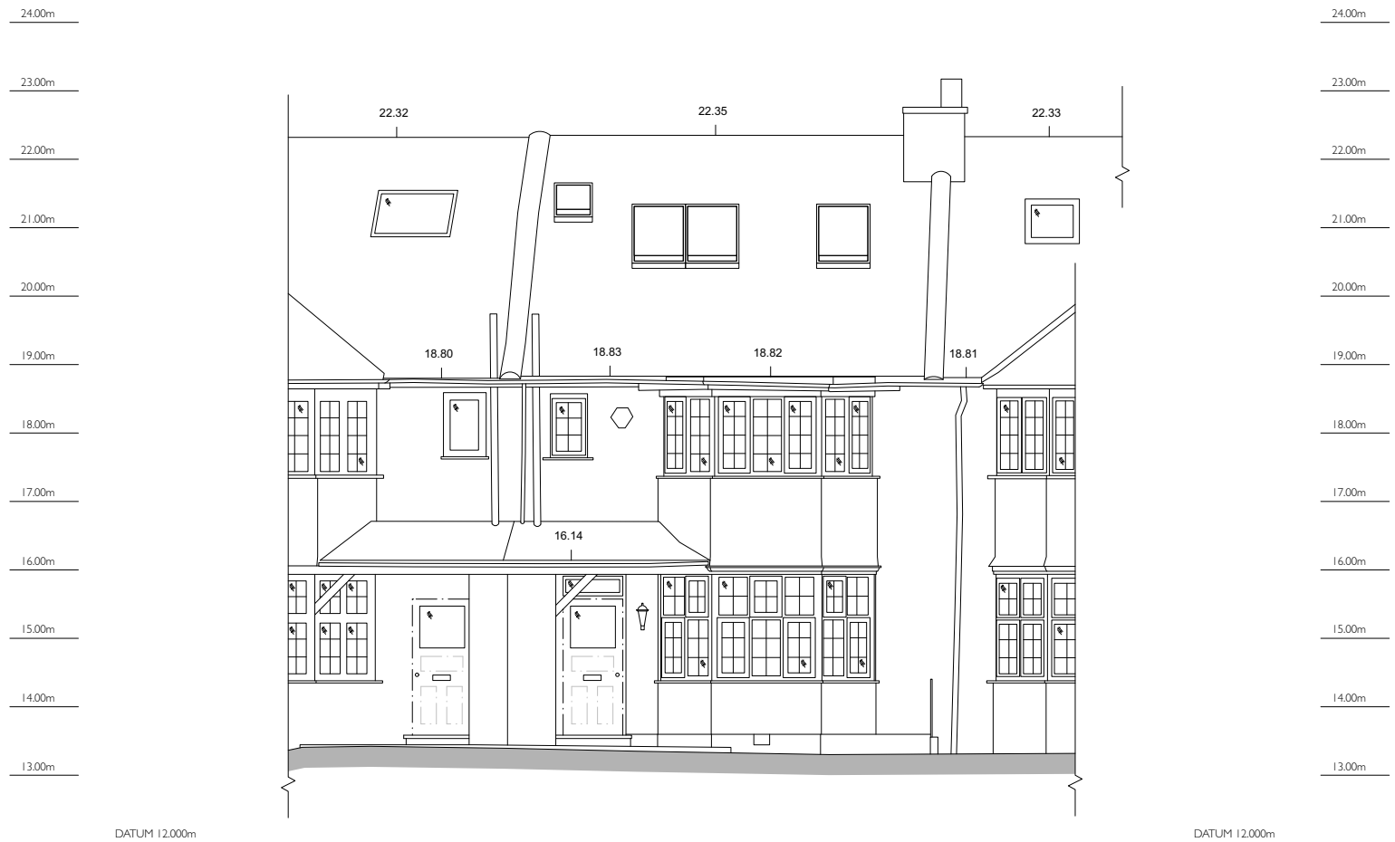
FRONT ELEVATION
